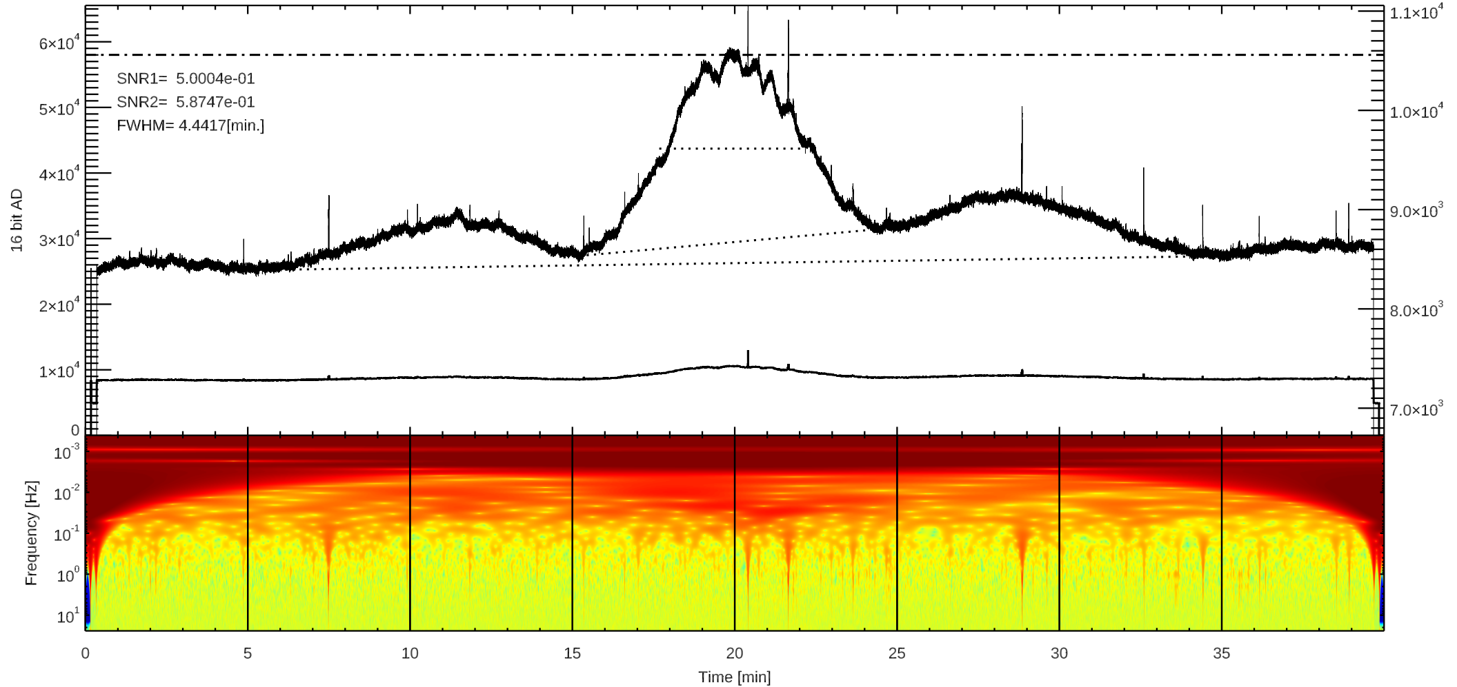
C 3C348 (/home4/archive/swift/dat/2025/03/T20250328040103.dat)
