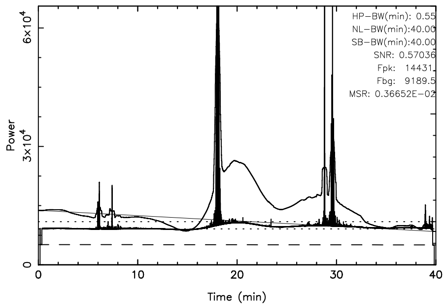
TOYOKAWA 3C348 2025/03/10(069)05:11:47-05:51:47JST
