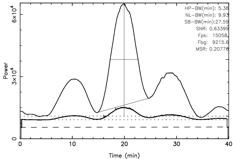
TOYOKAWA 3C274 2025/03/10(069)00:52:12-01:32:12JST
