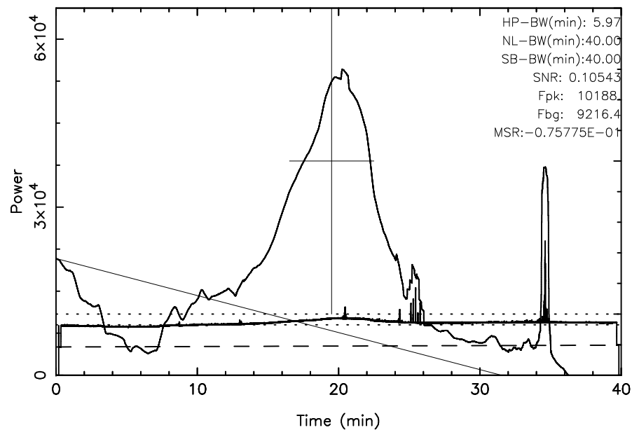
TOYOKAWA 3C295 2025/03/10(069)02:32:04-03:12:04JST
