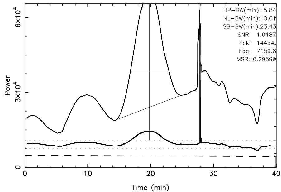
TOYOKAWA 3C144 2025/03/10(069)17:53:21-18:33:21JST
