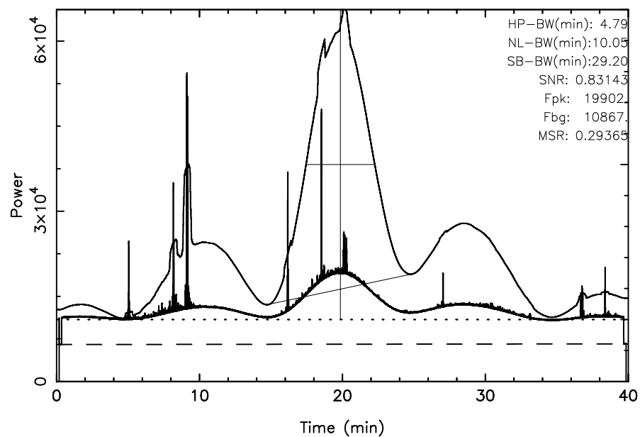
TOYOKAWA 3C274 2025/03/22(081)00:05:01-00:45:01JST
