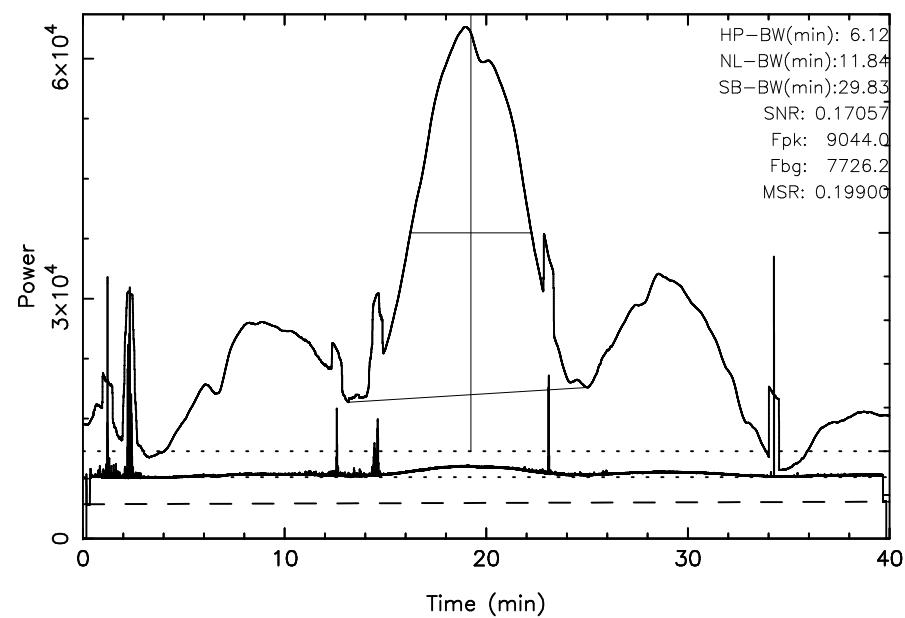
TOYOKAWA 3C157 2025/03/22(081)17:49:34-18:29:34JST
