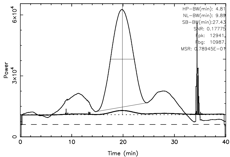
TOYOKAWA 3C348 2025/03/22(081)04:24:36-05:04:36JST
