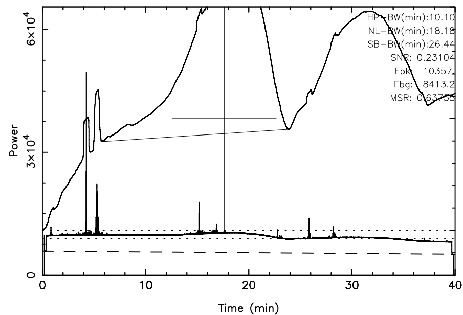
TOYOKAWA 3C295 2025/03/22(081)01:44:53-02:24:53JST
