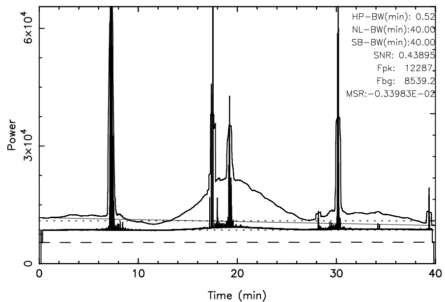
TOYOKAWA 3C295 2025/04/12(102)00:22:19-01:02:19JST
