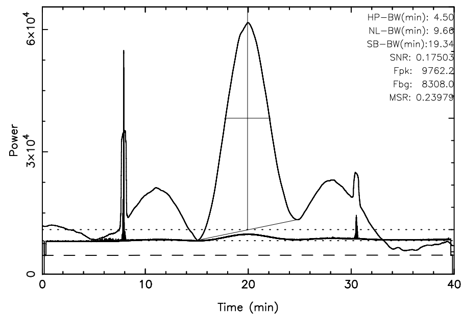
TOYOKAWA 3C348 2025/04/12(102)03:02:02-03:42:02JST
