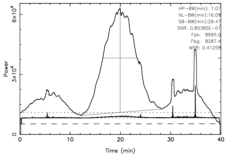
TOYOKAWA 3C295 2025/04/15(105)00:10:31-00:50:31JST
