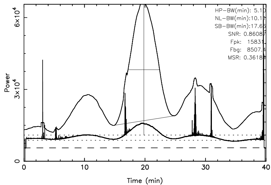
TOYOKAWA 3C274 2025/04/15(105)22:26:44-23:06:44JST
