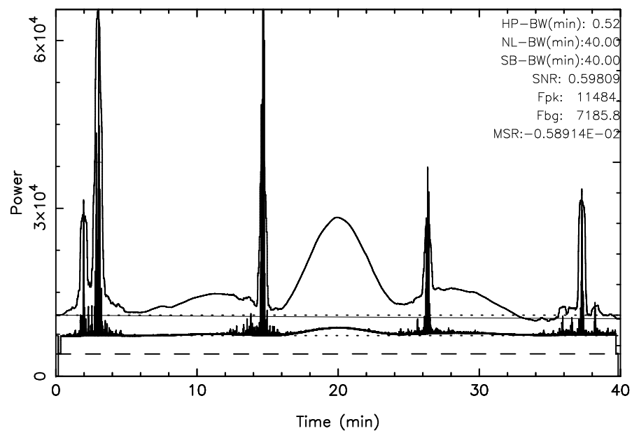
TOYOKAWA 3C348 2025/04/29(119)01:55:12-02:35:12JST
