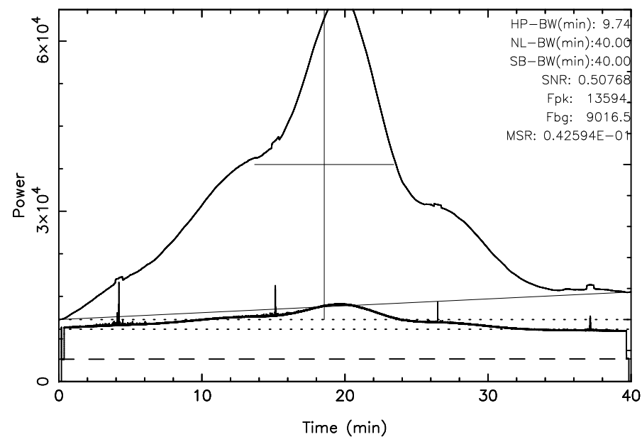
TOYOKAWA 3C392 2025/04/29(119)03:59:51-04:39:51JST
