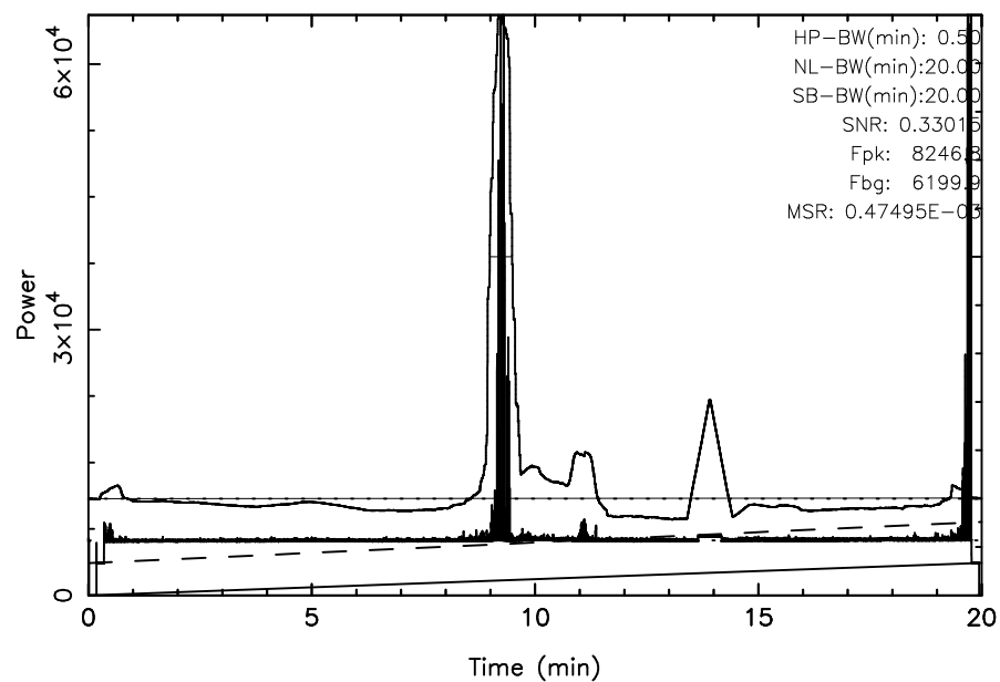
FUJI 3C348 2025/05/25(145)00:22:59-00:42:59JST
