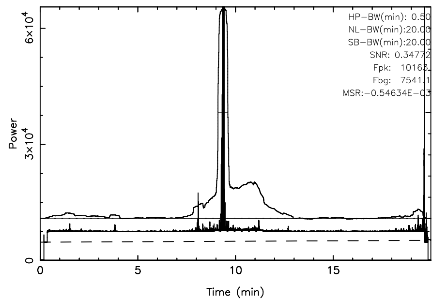
KISO 3C348 2025/05/25(145)00:22:59-00:42:59JST
