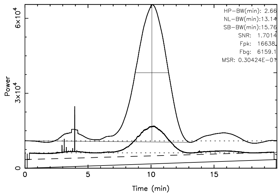
FUJI 3C405 2025/05/25(145)03:30:25-03:50:24JST
