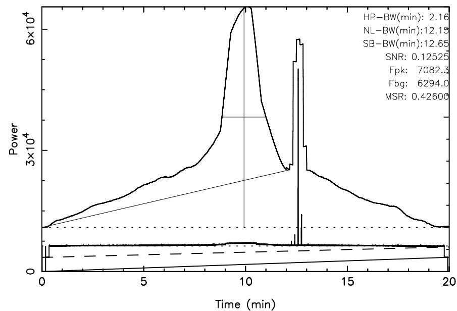
FUJI 3C392 2025/05/25(145)02:27:37-02:47:37JST
