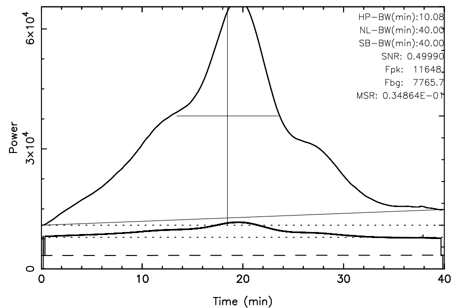
TOYOKAWA 3C392 2025/05/04(124)03:40:11-04:20:11JST
