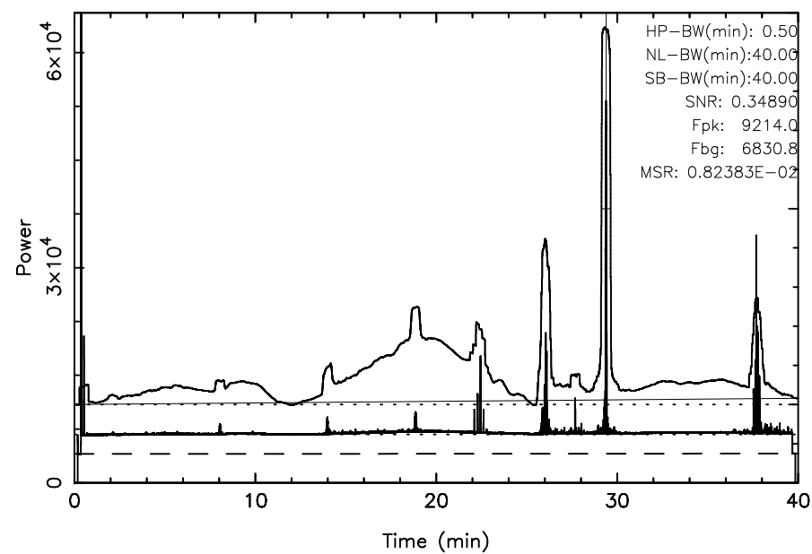
TOYOKAWA 3C295 2025/05/04(124)22:51:53-23:31:53JST
