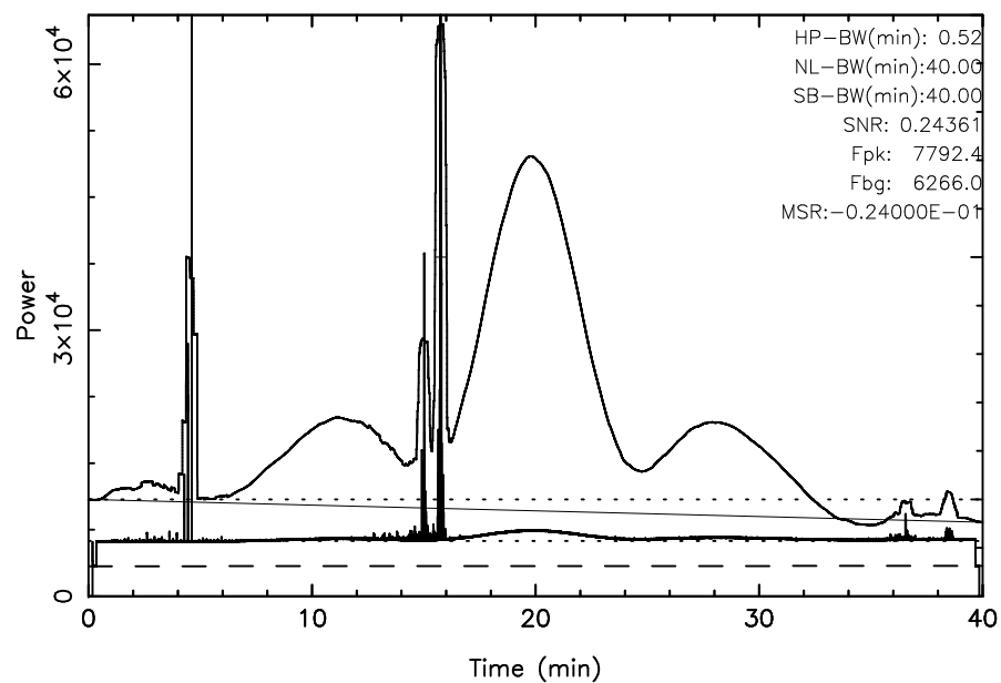
TOYOKAWA 3C348 2025/05/04(124)01:35:33-02:15:33JST
