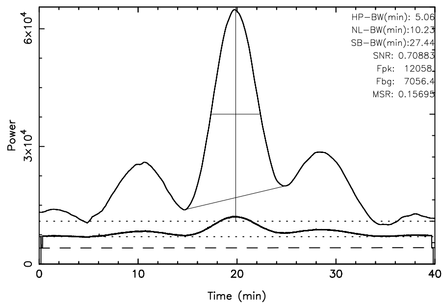
TOYOKAWA 3C274 2025/05/04(124)21:12:02-21:52:02JST
