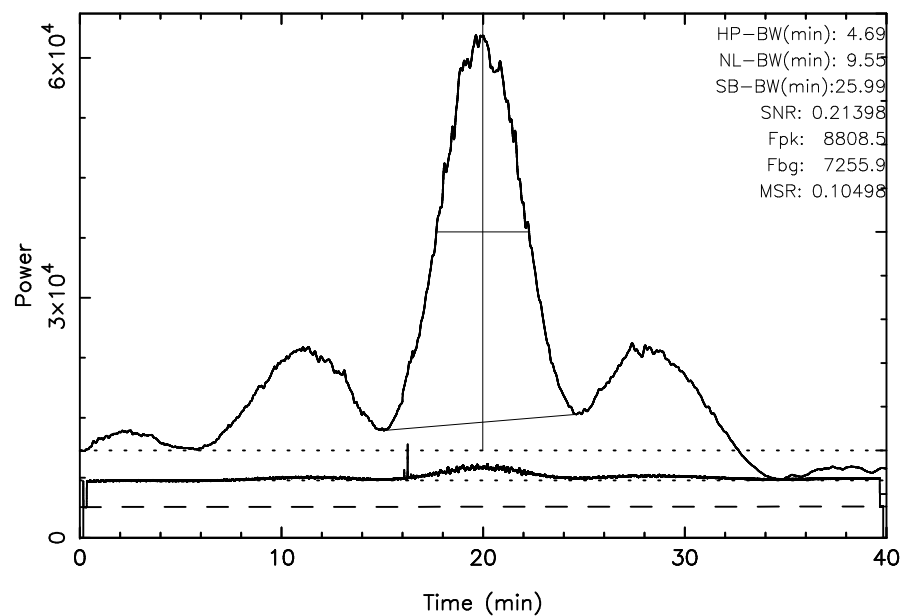
TOYOKAWA 3C348 2025/05/13(133)01:00:09–01:40:09JST
