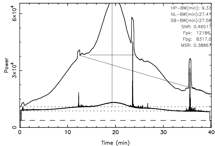
TOYOKAWA 3C392 2025/05/13(133)03:04:48–03:44:48JST
