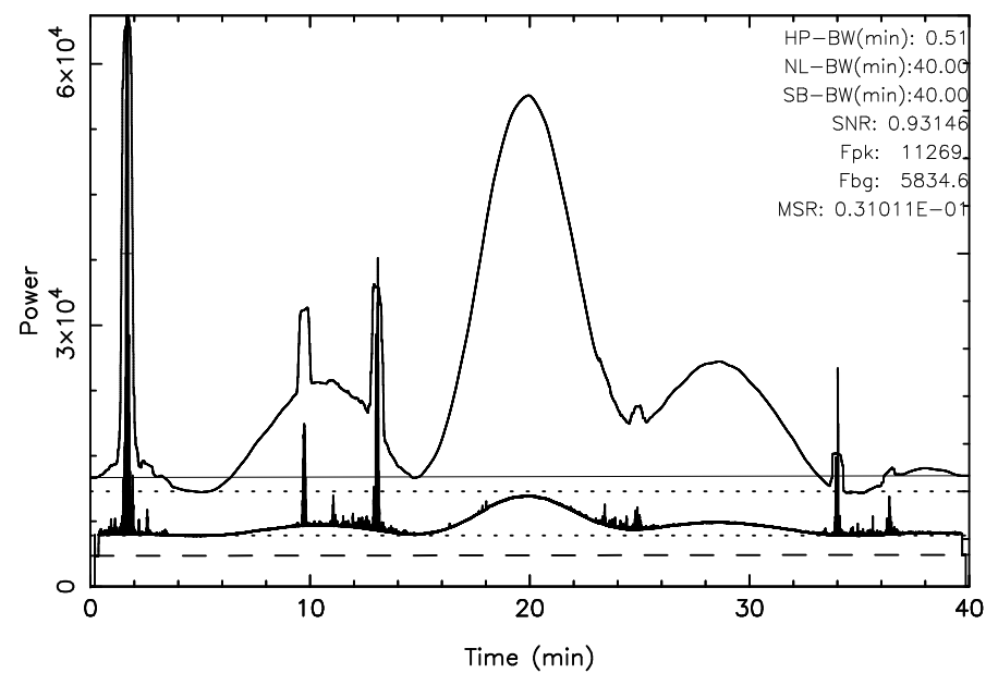
TOYOKAWA 3C274 2025/05/13(133)20:36:39–21:16:39JST
