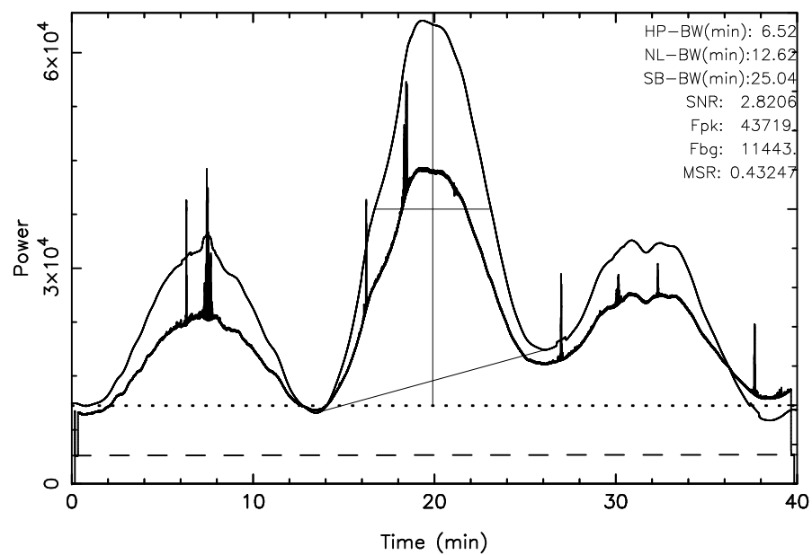
TOYOKAWA 3C405 2025/05/13(133)04:07:36–04:47:36JST
