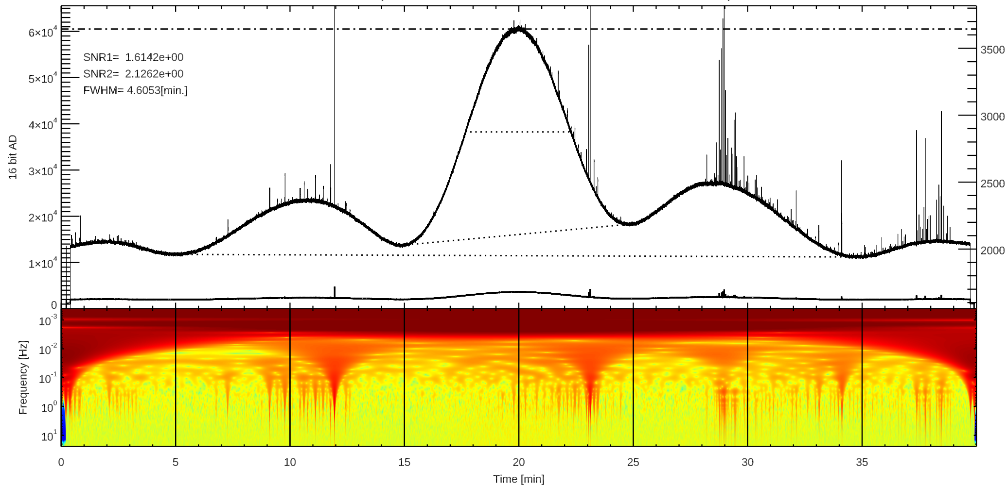
C 3C274 (/home4/archive/swift/dat/2023/05/T20230503211807.dat)
