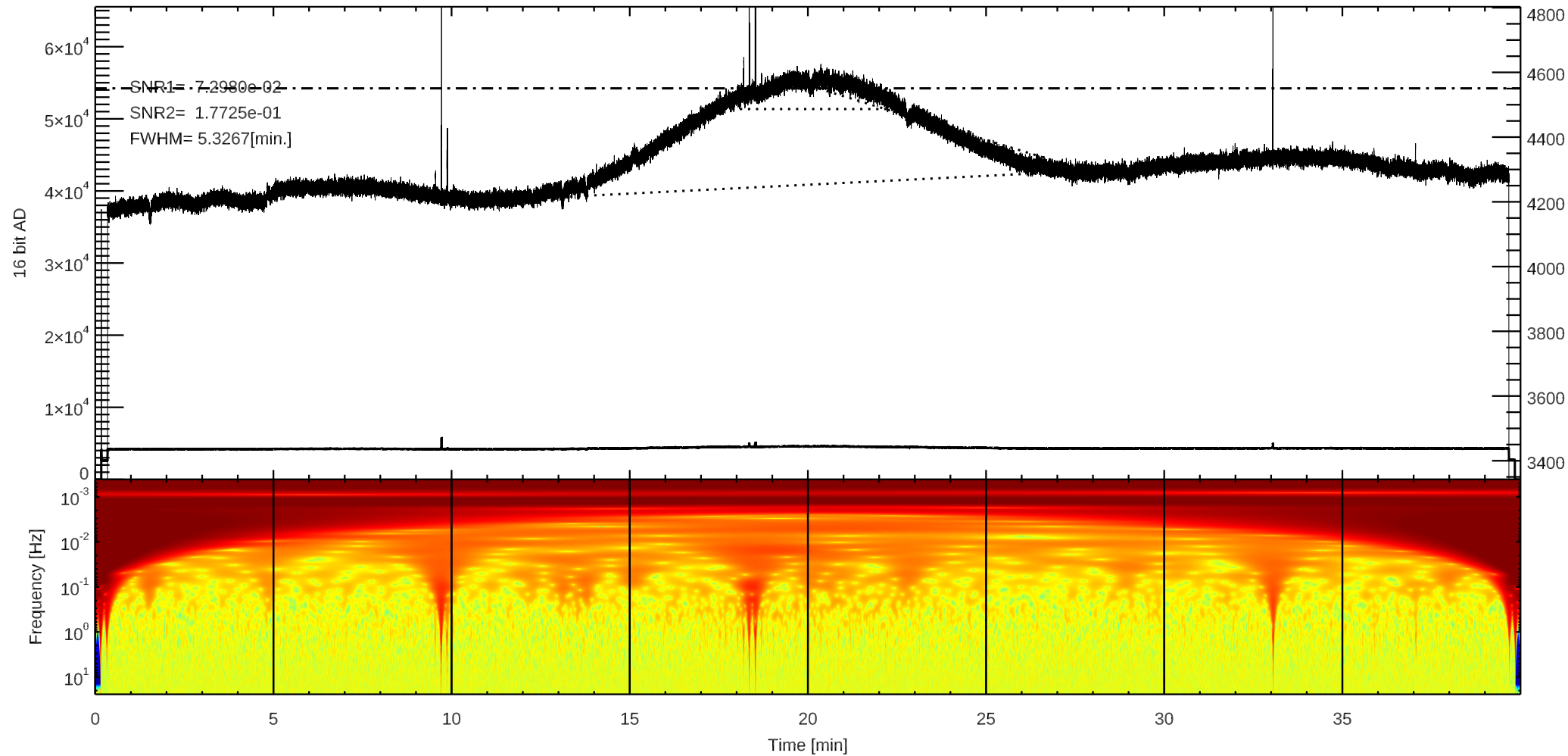
C 3C295 (/home4/archive/swift/dat/2025/06/T20250616200251.dat)
