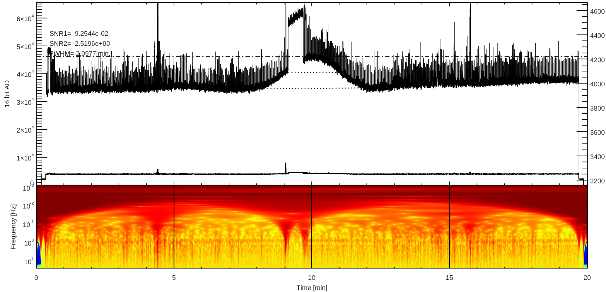
C 3C348 (/home4/archive/fit/dat/2025/06/F20250630215731.dat)
