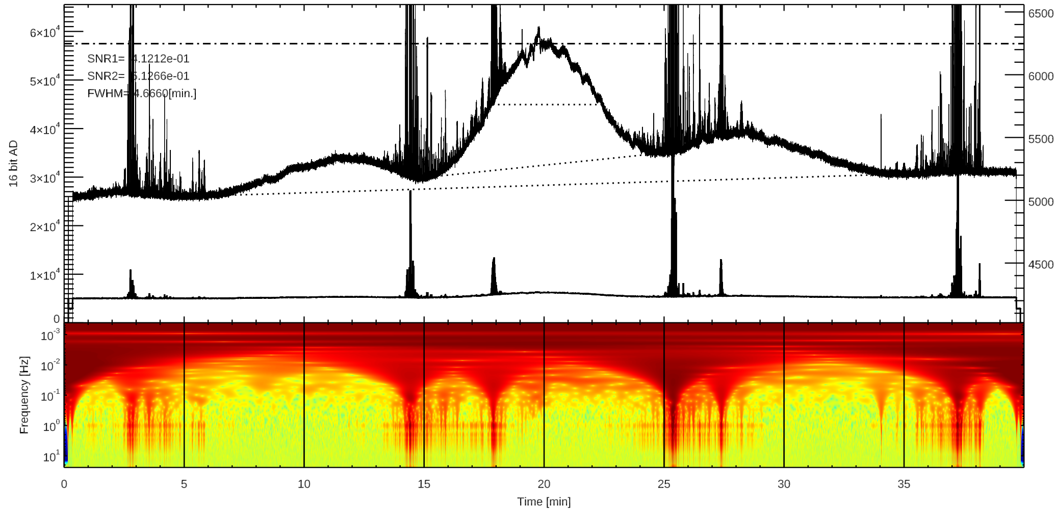
C 3C348 (/home4/archive/swift/dat/2025/06/T20250617223839.dat)
