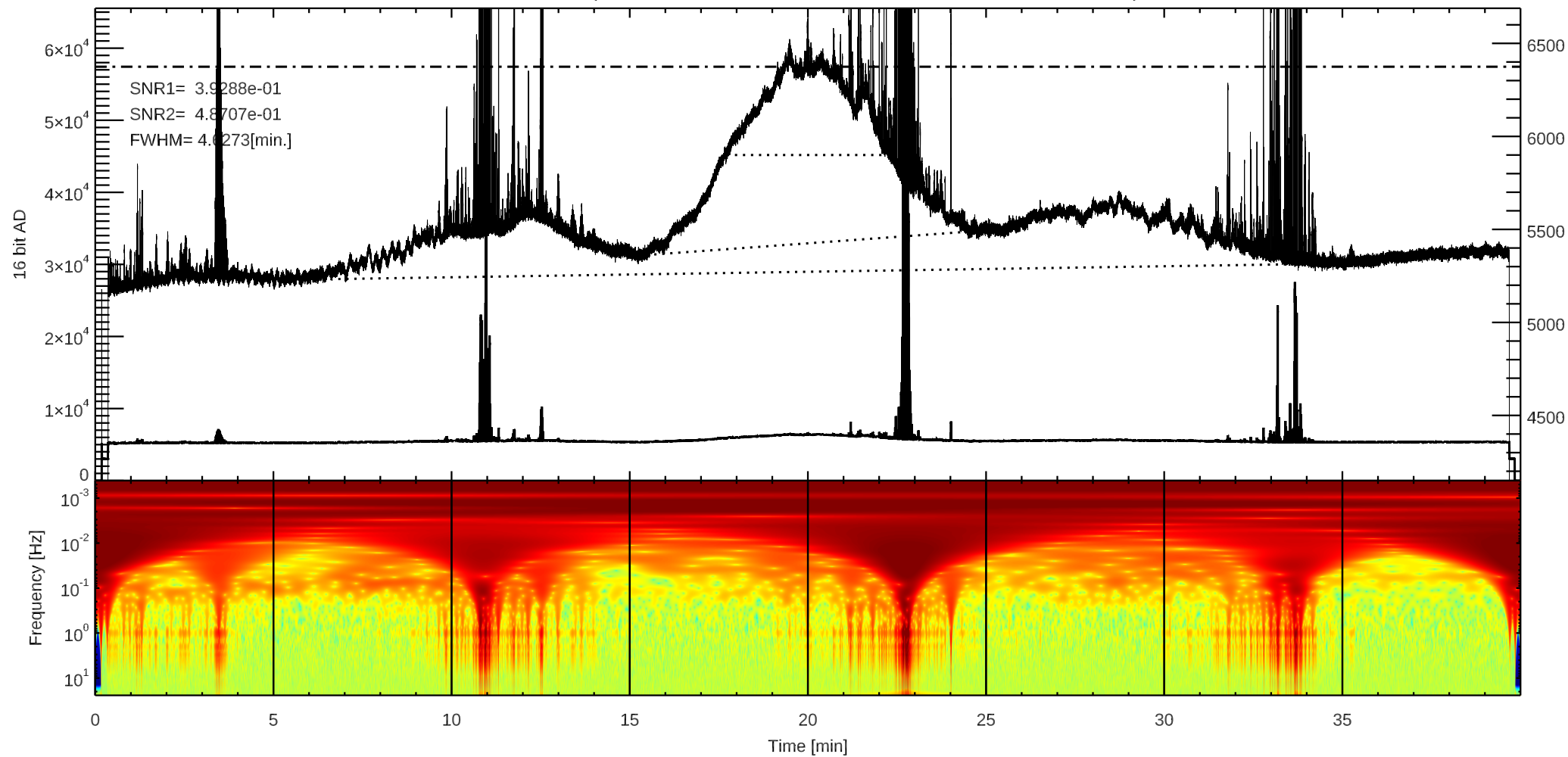
C 3C348 (/home4/archive/swift/dat/2025/06/T20250618223443.dat)
