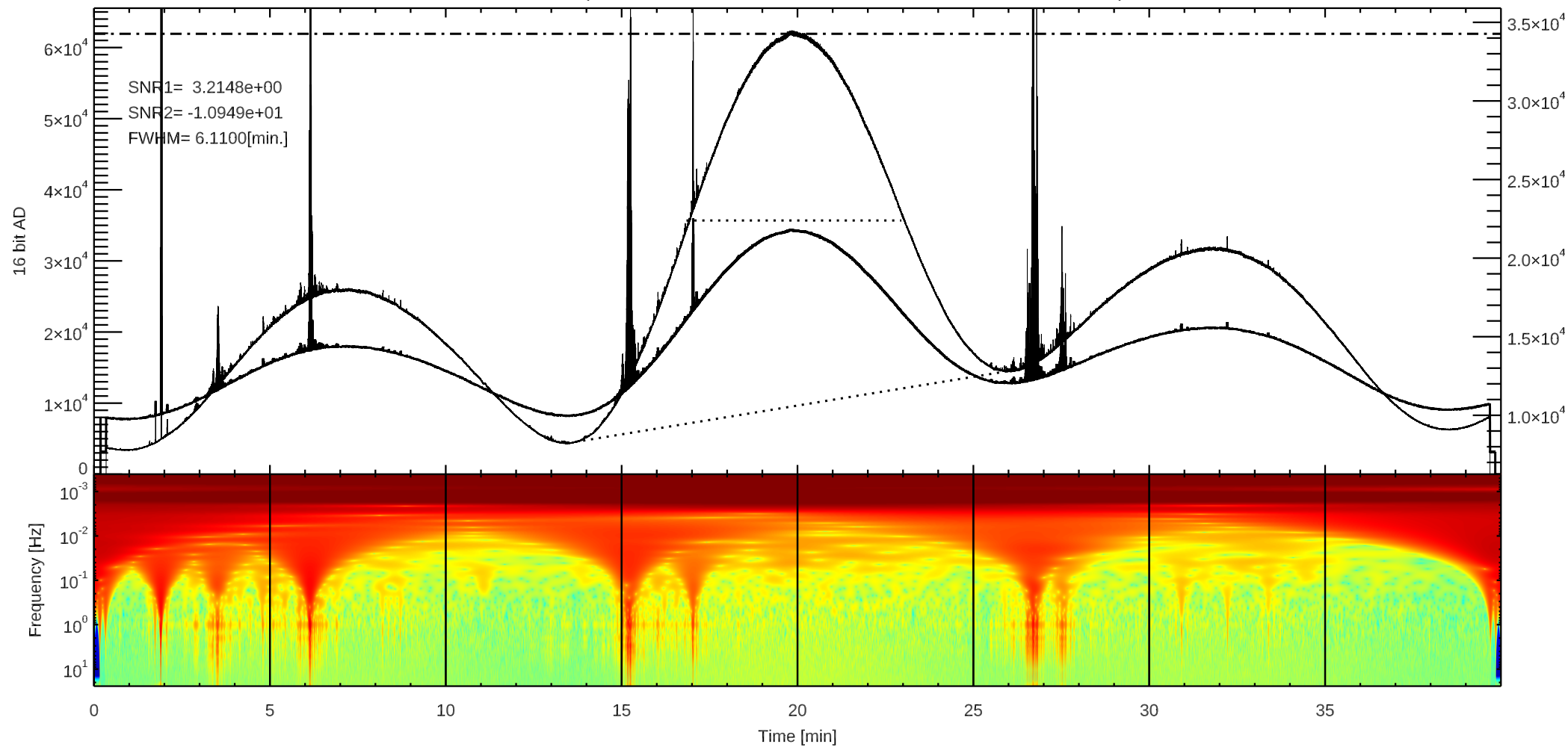
C 3C405 (/home4/archive/swift/dat/2025/06/T20250614020149.dat)
