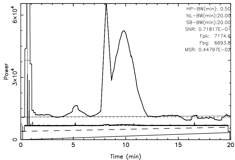
FUJI 3C353 2025/05/31(151)00:28:44-00:48:44JST
