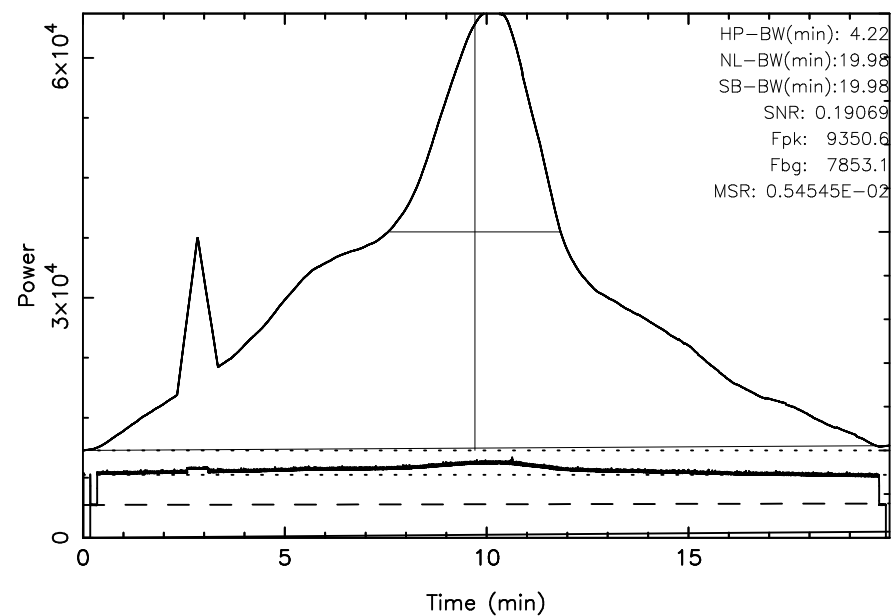
FUJI 3C392 2025/05/31(151)02:04:02-02:24:01JST
