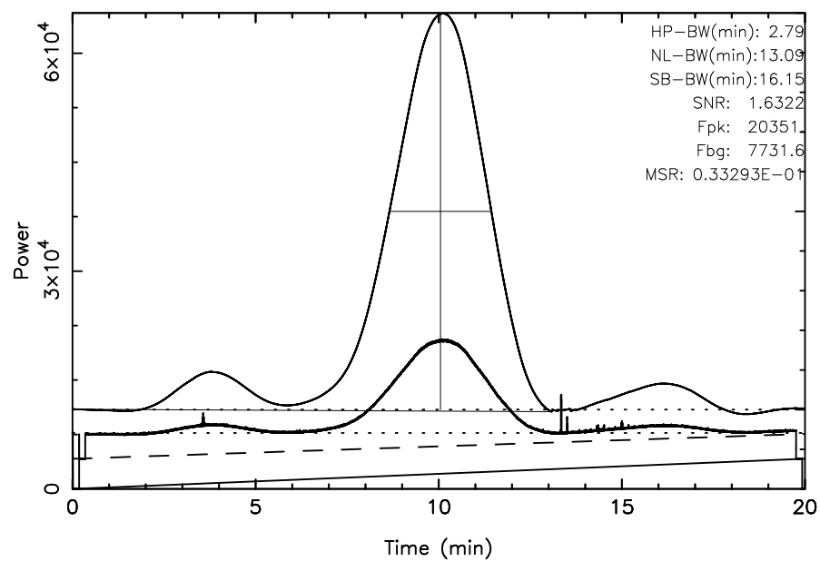
FUJI 3C405 2025/05/31(151)03:06:50-03:26:50JST
