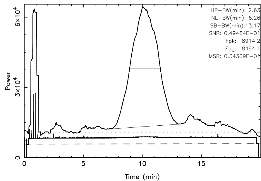
KISO 3C353 2025/05/31(151)00:28:44-00:48:44JST
