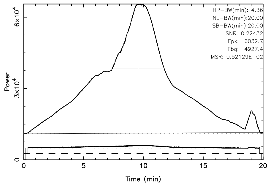
FUJI 3C392 2025/06/27(178)00:17:52-00:37:52JST
