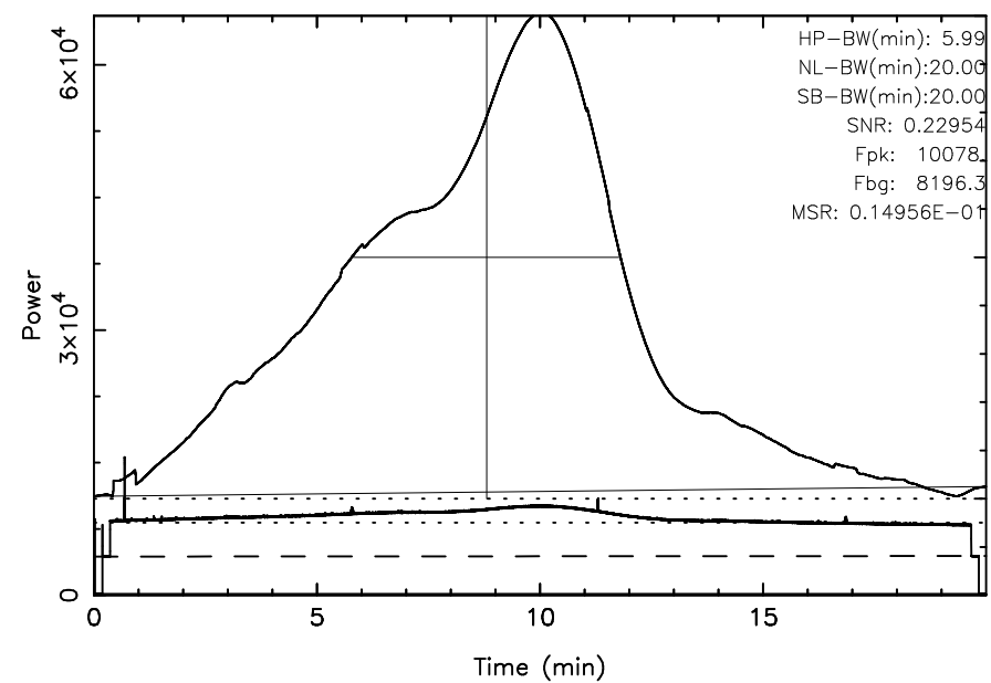
KISO 3C392 2025/06/27(178)00:17:52-00:37:52JST
