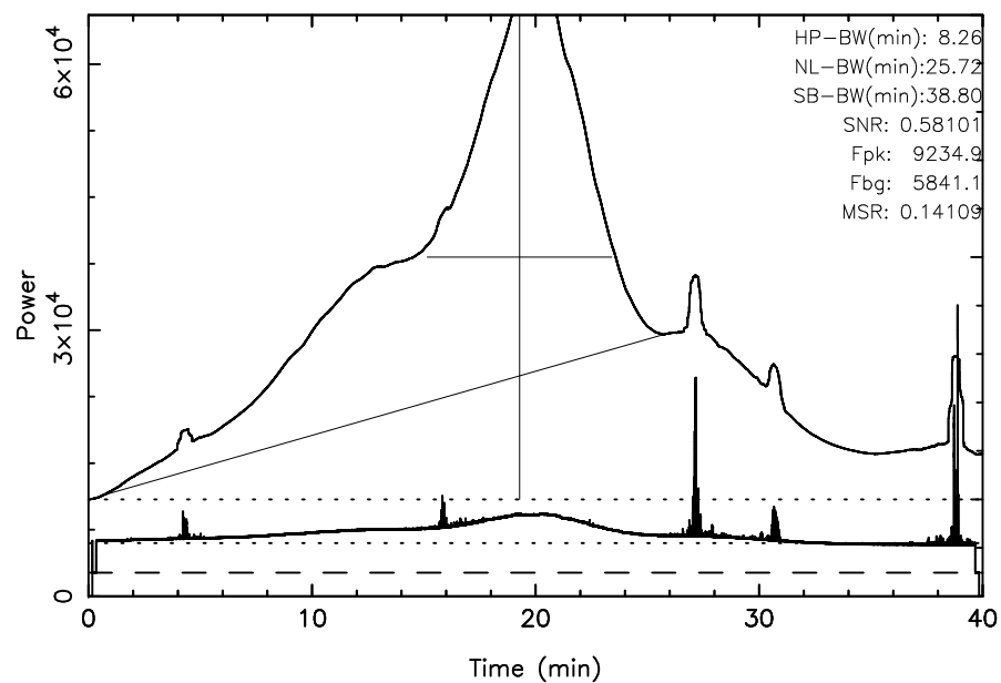
TOYOKAWA 3C392 2025/06/11(162)01:10:47-01:50:47JST
