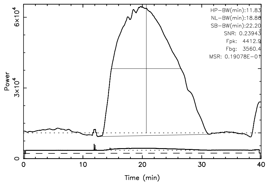
TOYOKAWA 3C295 2025/06/11(162)20:22:29-21:02:29JST
