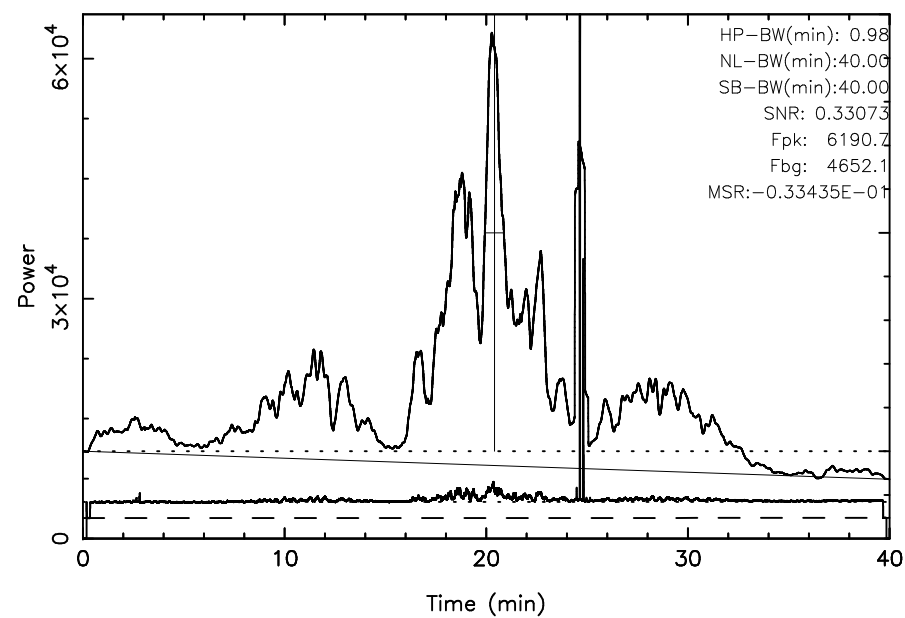
TOYOKAWA 3C348 2025/06/11(162)23:02:12-23:42:12JST
