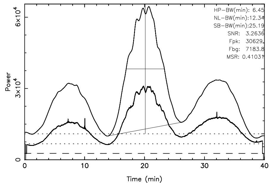
TOYOKAWA 3C405 2025/06/11(162)02:13:35-02:53:35JST
