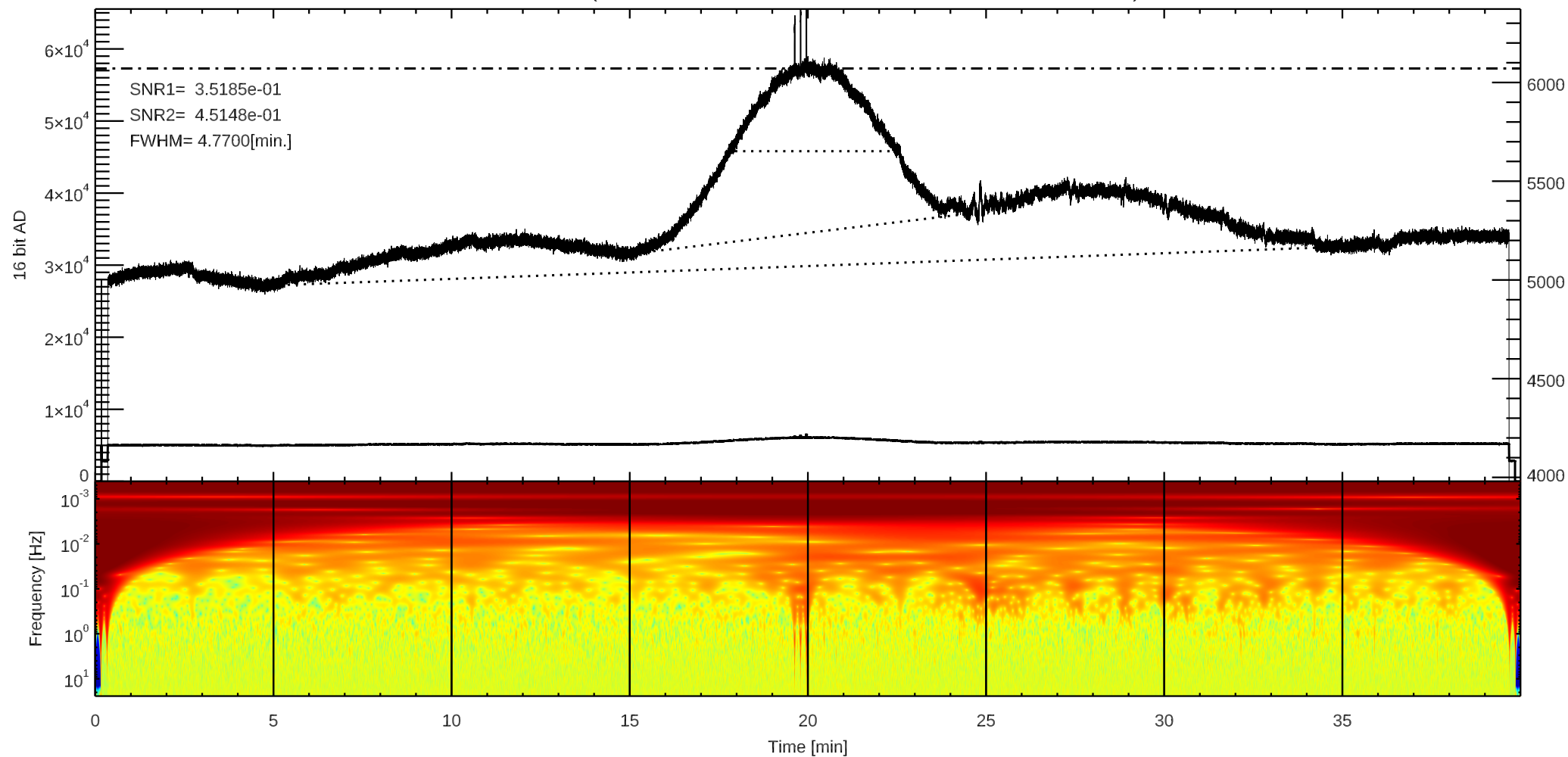
C 3C348 (/home4/archive/swift/dat/2025/07/T20250706212357.dat)
