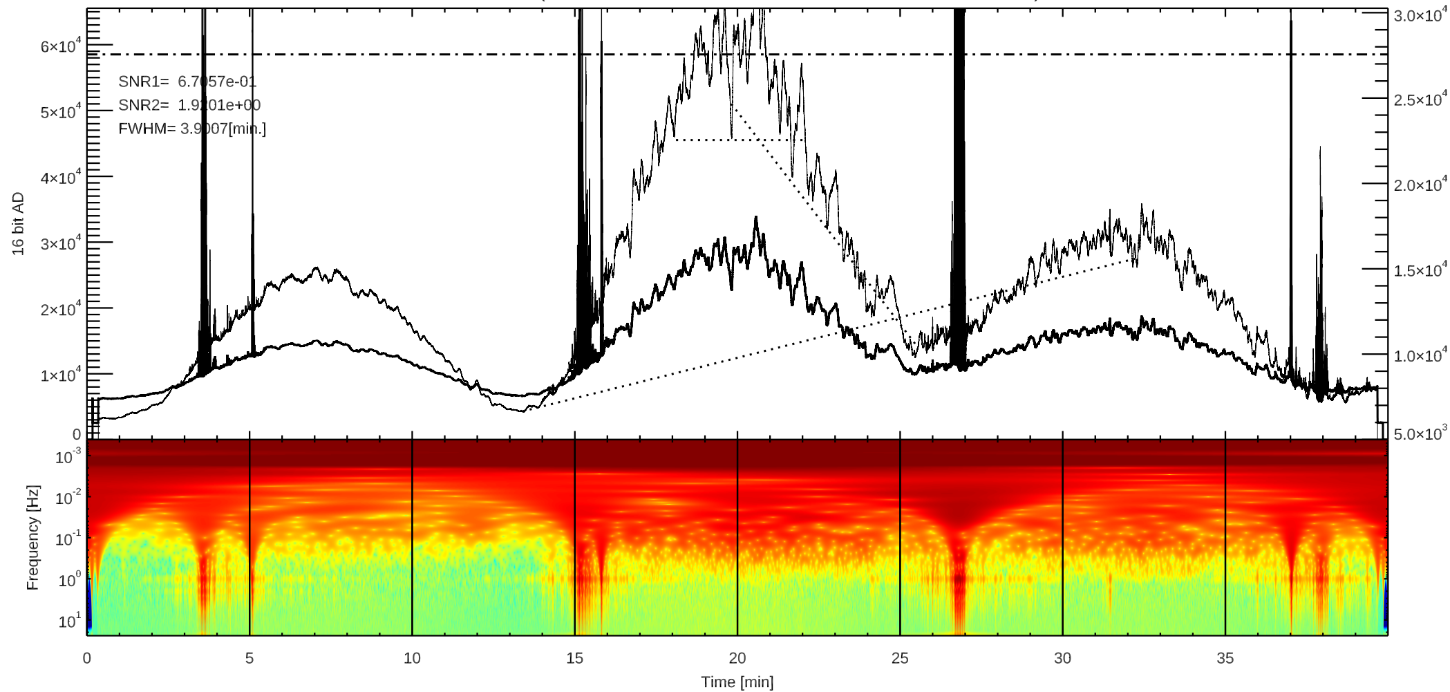
C 3C405 (/home4/archive/swift/dat/2025/07/T20250704004311.dat)
