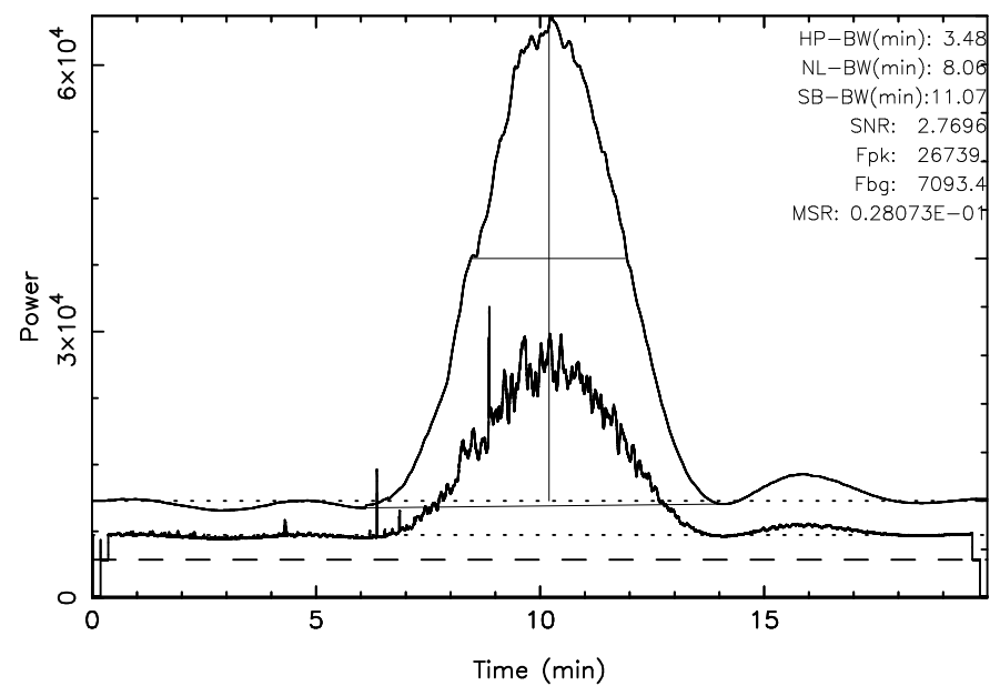
KISO 3C405 2025/07/11(192)00:25:38–00:45:37JST
