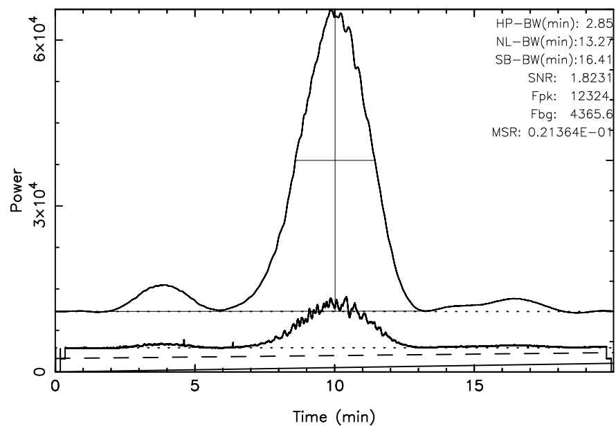
FUJI 3C405 2025/07/11(192)00:25:38–00:45:37JST
