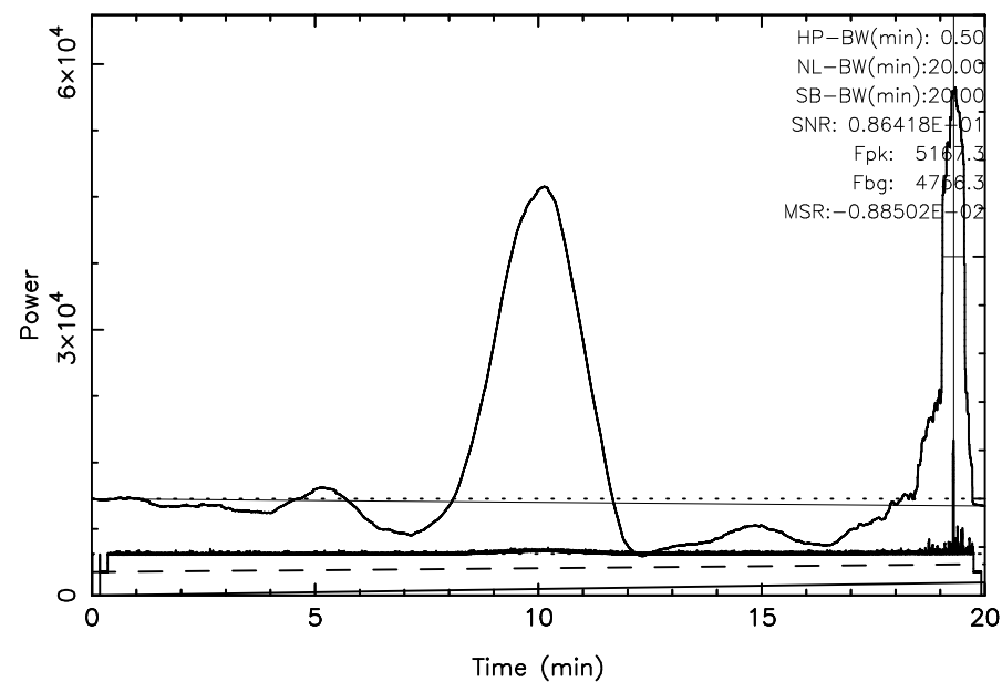
FUJI 3C348 2025/07/11(192)21:14:15–21:34:15JST
