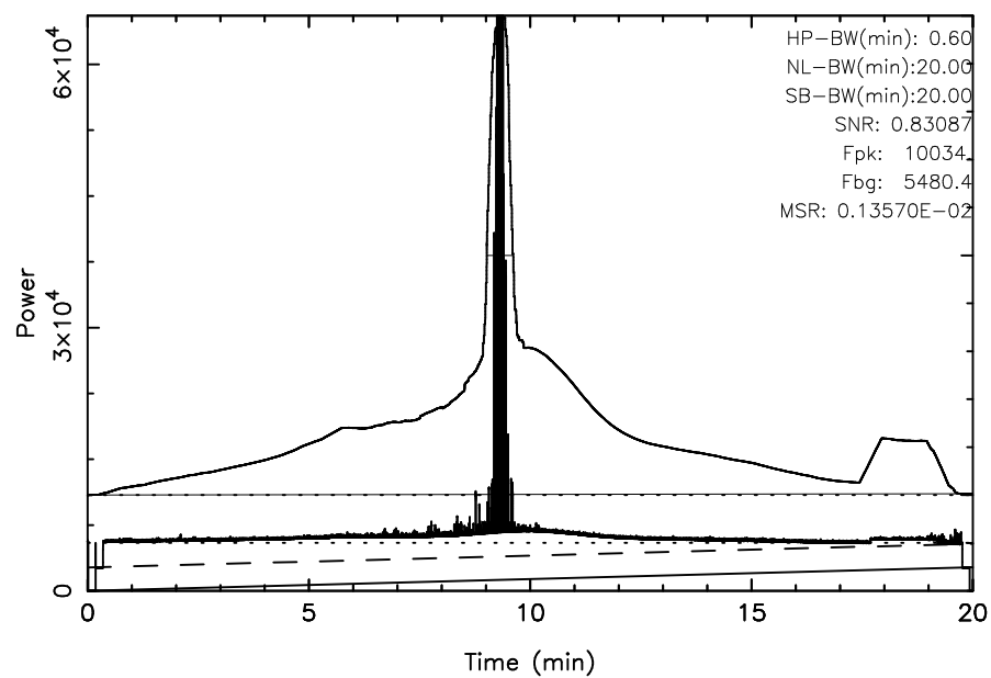
FUJI 3C392 2025/07/11(192)23:18:54–23:38:54JST
