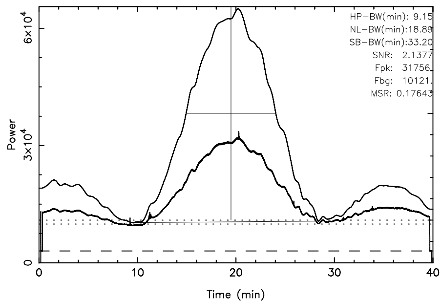
TOYOKAWA 3C461 2025/07/24(205)02:48:08–03:28:08JST
