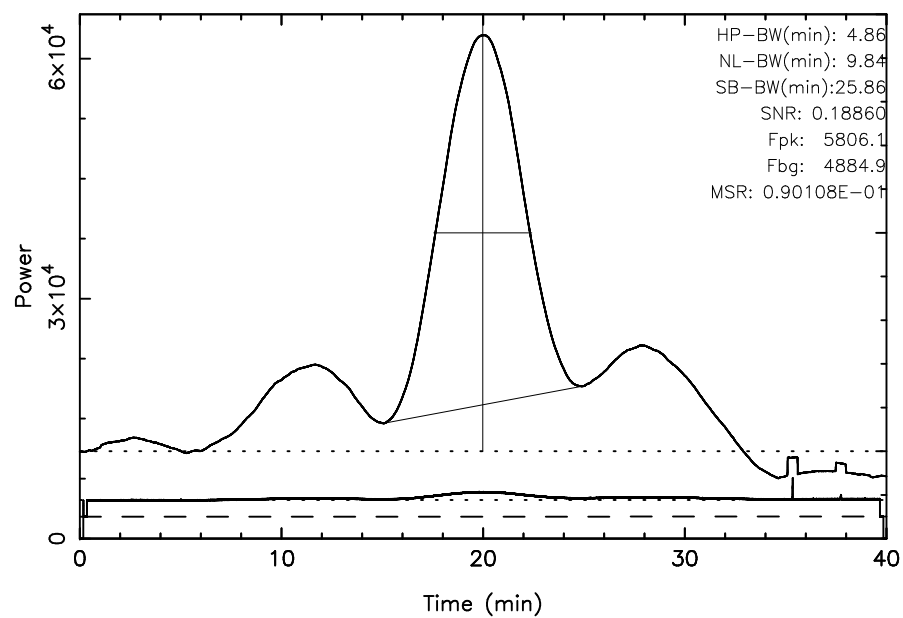
TOYOKAWA 3C348 2025/07/24(205)20:13:09–20:53:09JST
