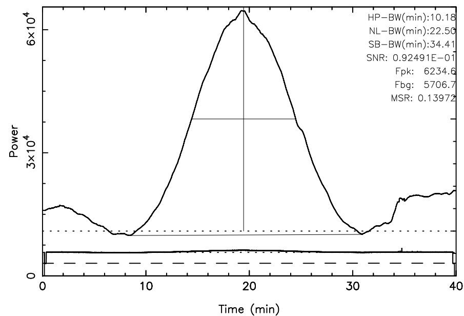
TOYOKAWA 3C10 2025/07/24(205)03:50:17–04:30:17JST
