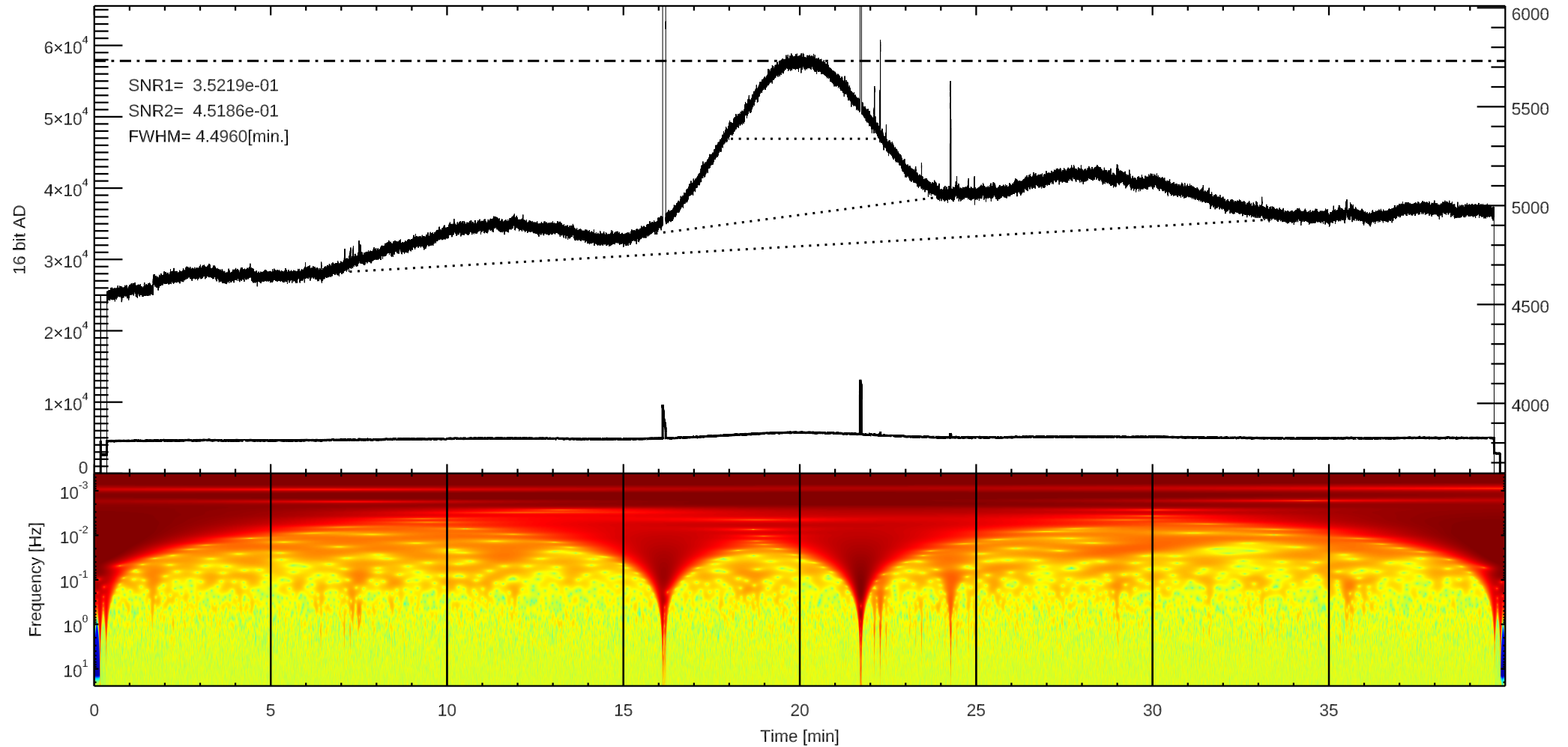
C 3C348 (/home4/archive/swift/dat/2025/08/T20250819183057.dat)
