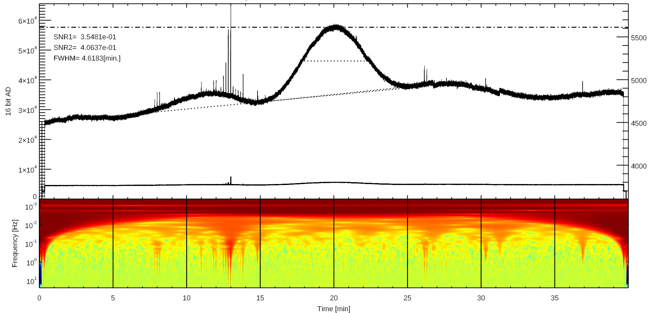
C 3C348 (/home4/archive/swift/dat/2025/08/T20250823181514.dat)
