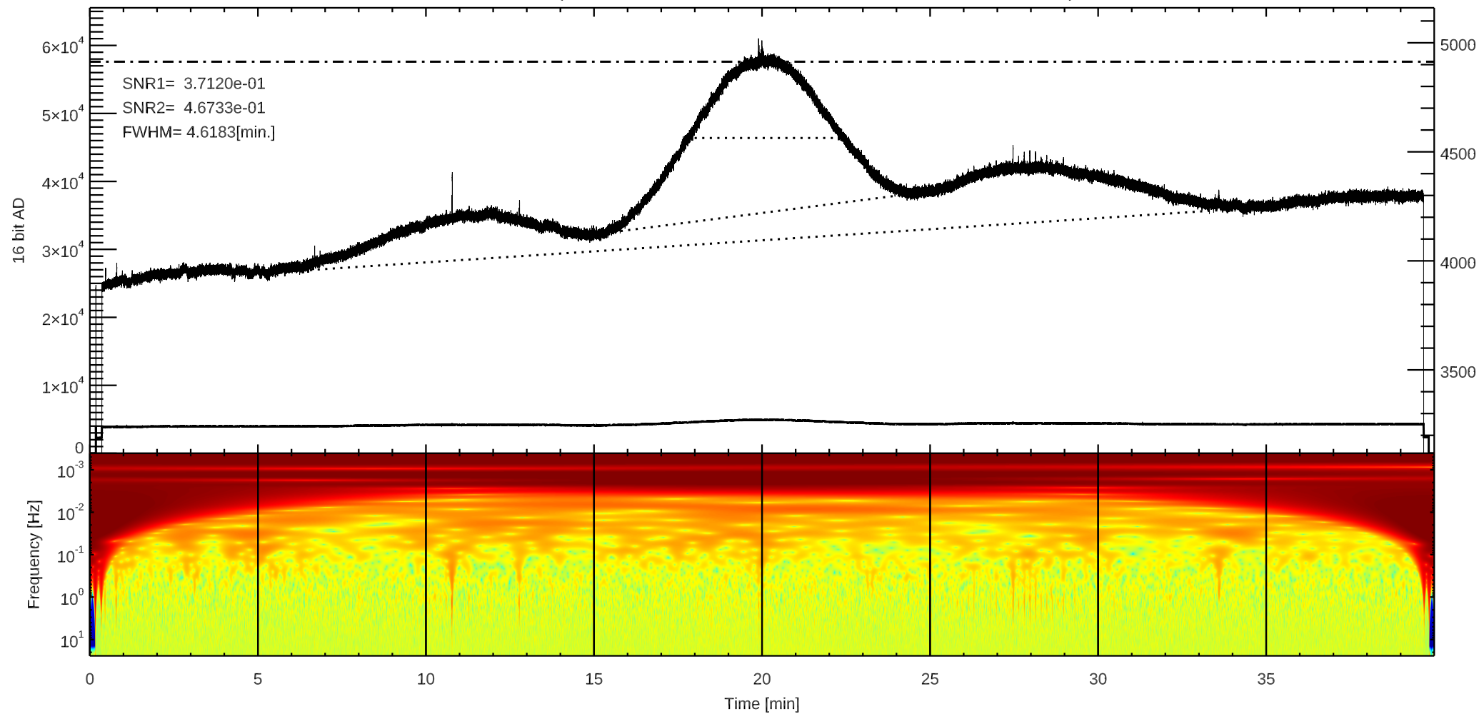
C 3C348 (/home4/archive/swift/dat/2025/08/T20250826180326.dat)
