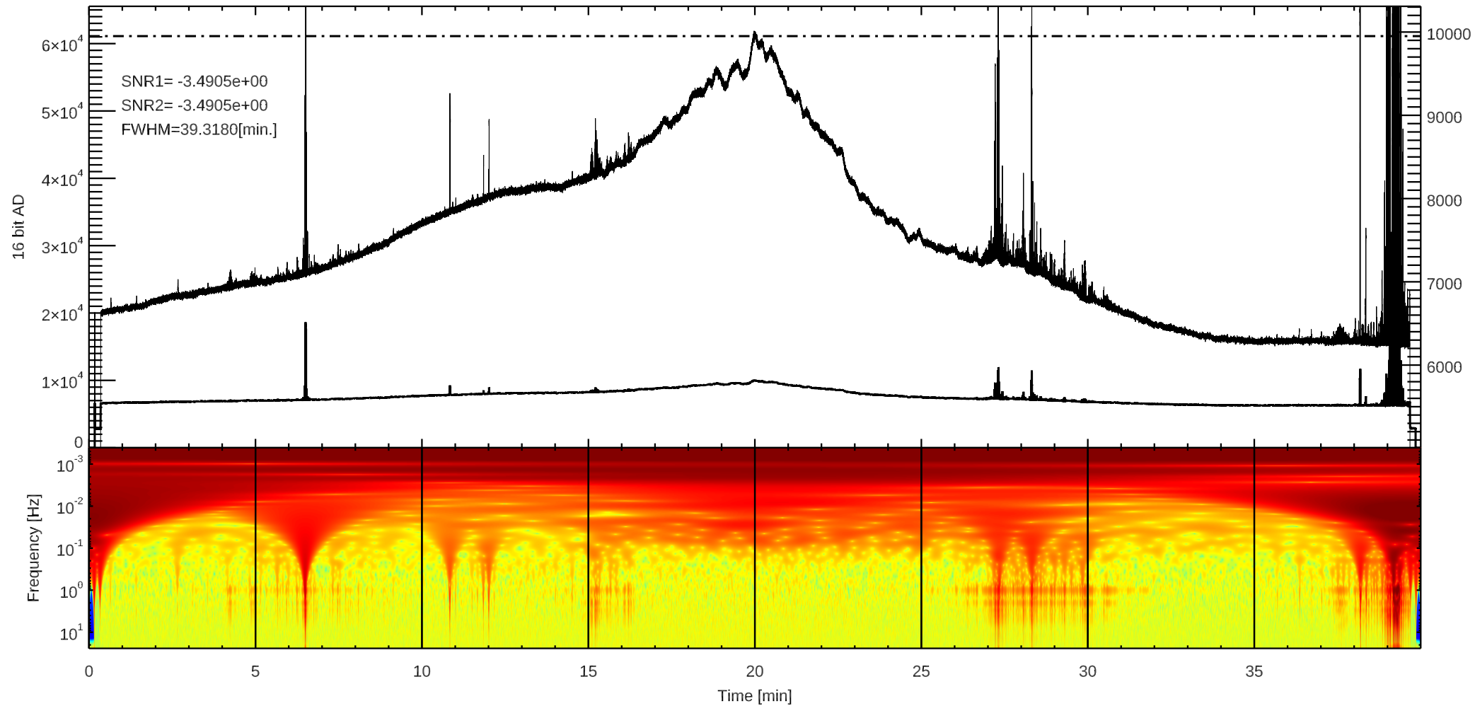
C 3C392 (/home4/archive/swift/dat/2025/08/T20250801214622.dat)
