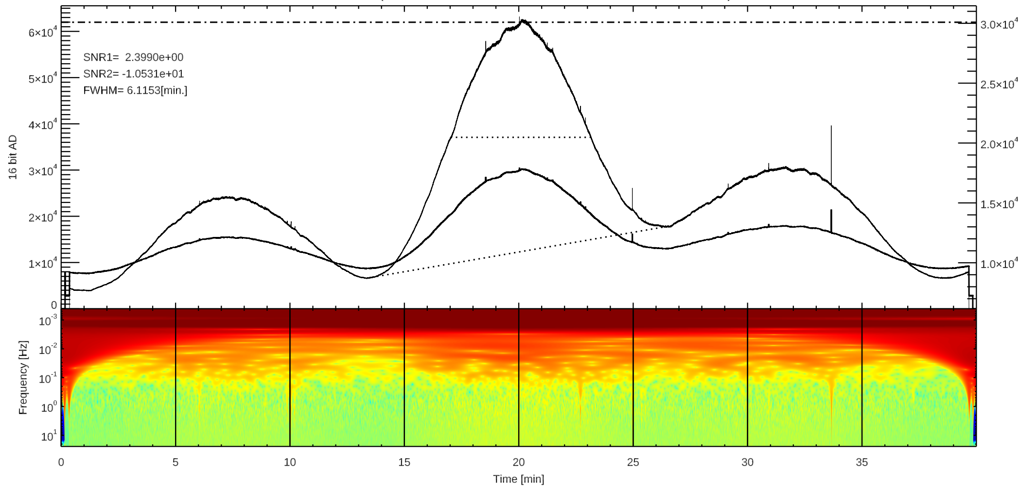
C 3C405 (/home4/archive/swift/dat/2025/08/T20250816215011.dat)
