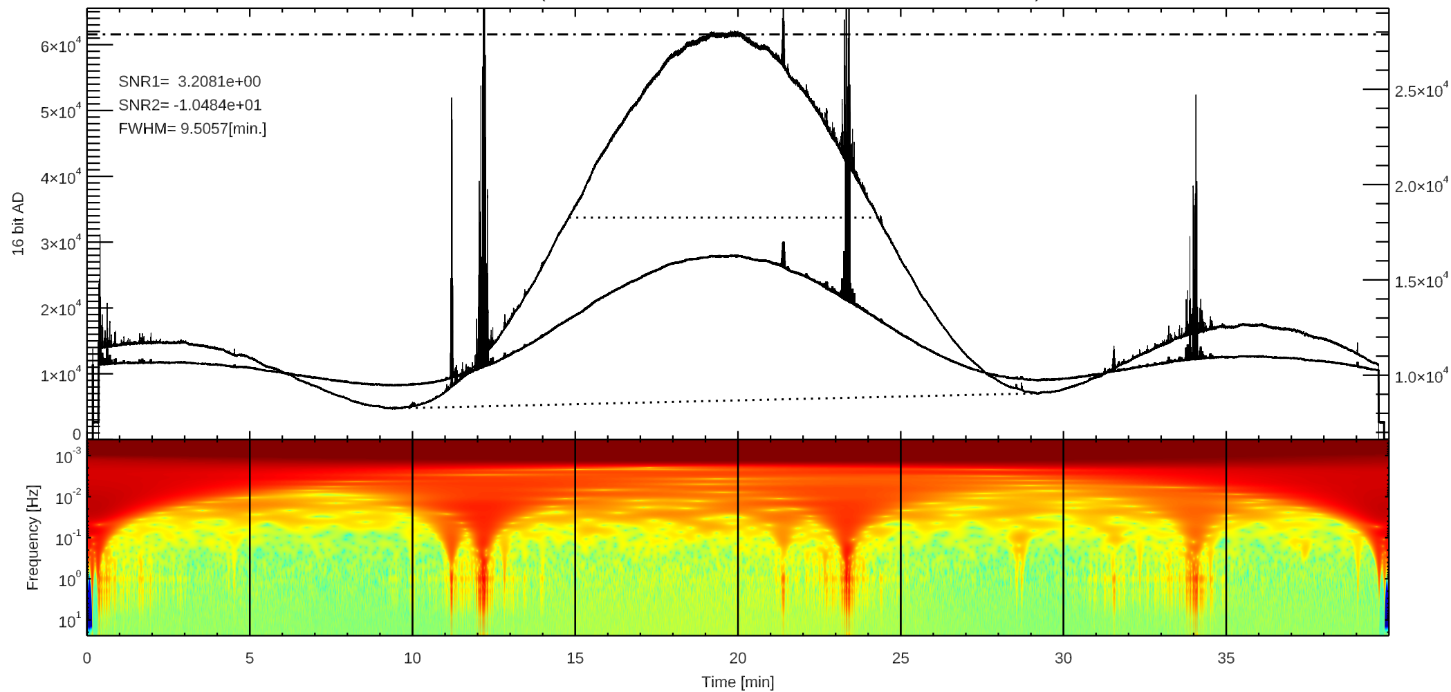
C 3C461 (/home4/archive/swift/dat/2025/08/T20250813012932.dat)
