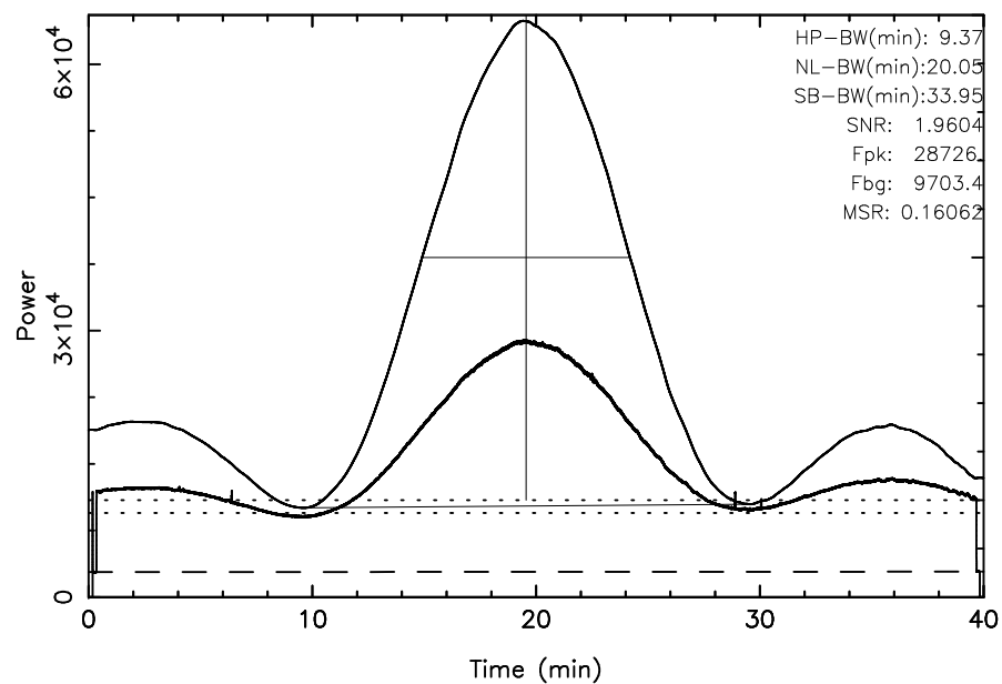
TOYOKAWA 3C461 2025/08/05(217)02:00:57-02:40:57JST
