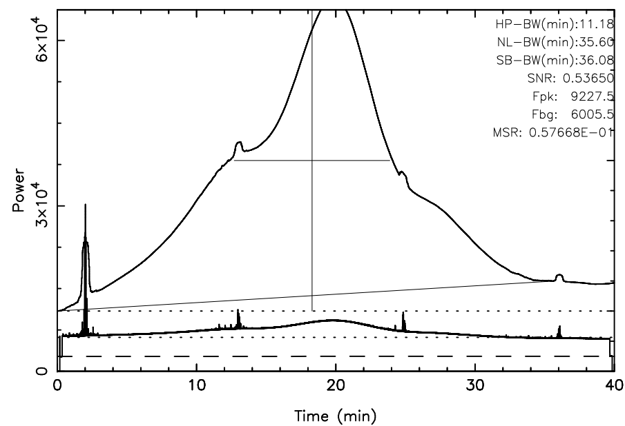
TOYOKAWA 3C392 2025/08/05(217)21:30:37-22:10:37JST
