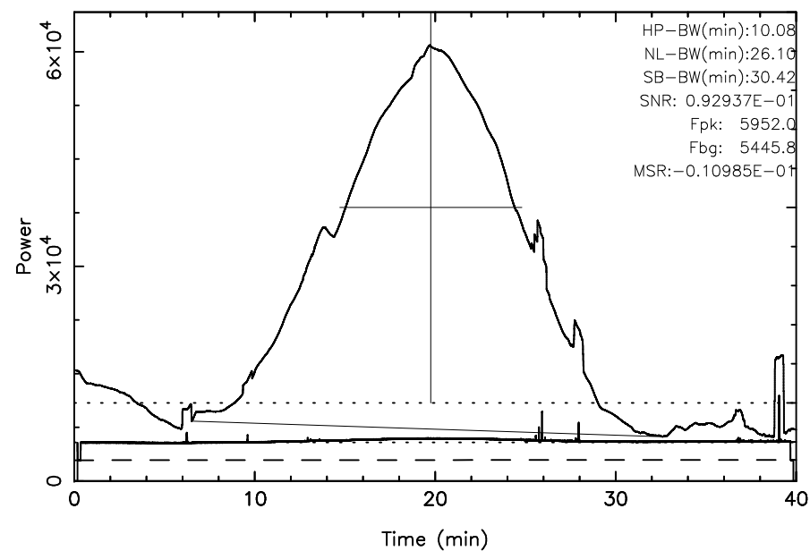
TOYOKAWA 3C10 2025/08/05(217)03:03:06-03:43:06JST
