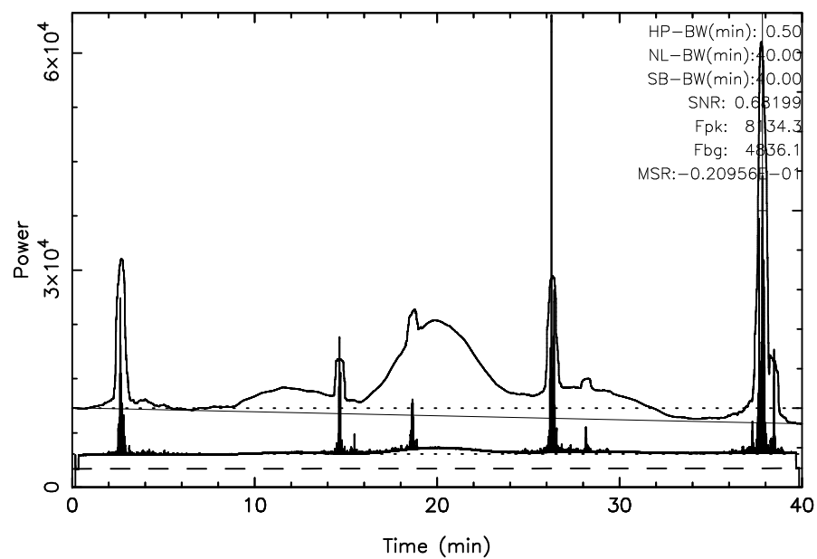
TOYOKAWA 3C348 2025/08/05(217)19:25:58-20:05:58JST
