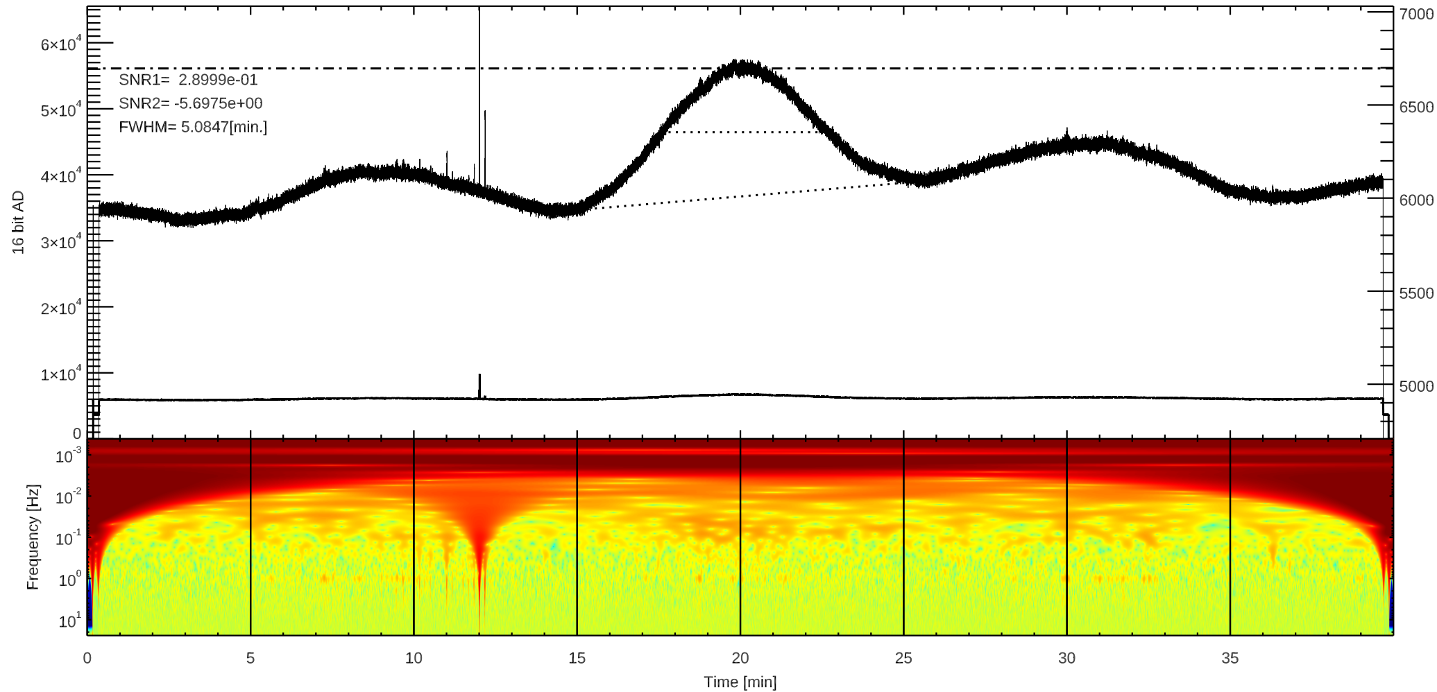
C 3C123 (/home4/archive/swift/dat/2025/09/T20250924035742.dat)
