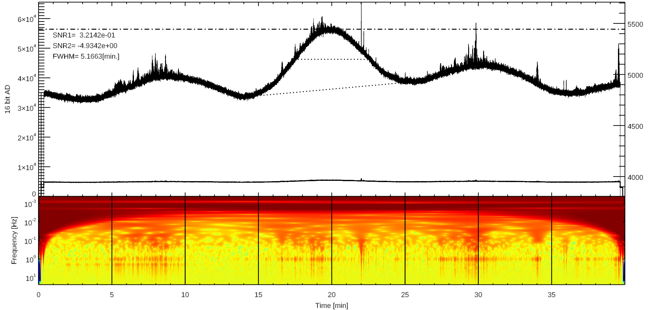
C 3C123 (/home4/archive/swift/dat/2025/09/T20250929033803.dat)
