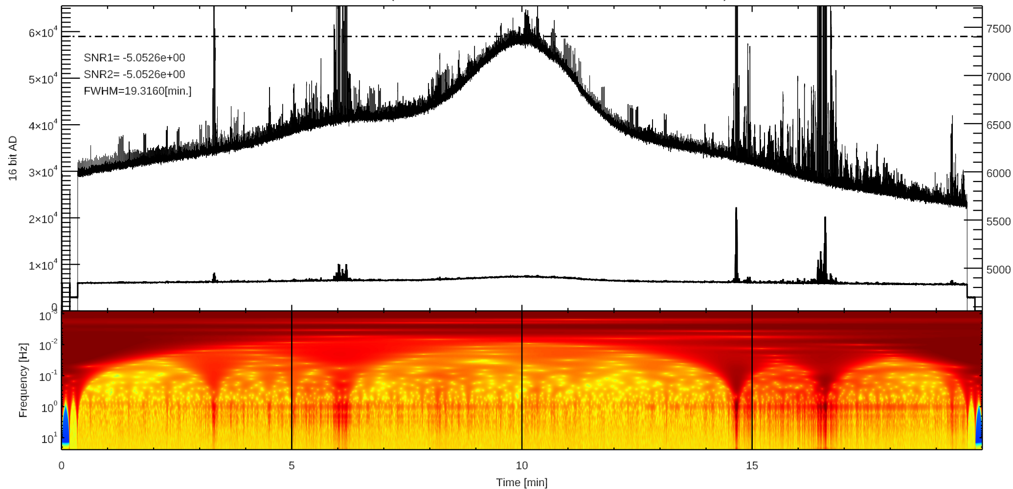
C 3C392 (/home4/archive/fit/dat/2025/09/F20250919184343.dat)
