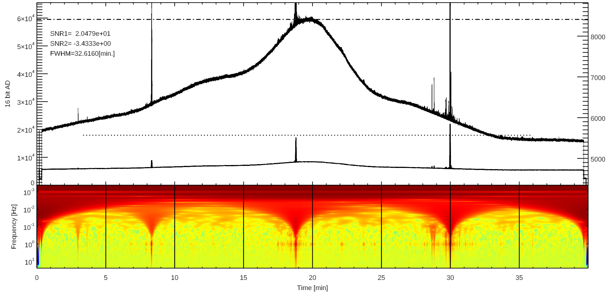
C 3C392 (/home4/archive/swift/dat/2025/09/T20250917184135.dat)
