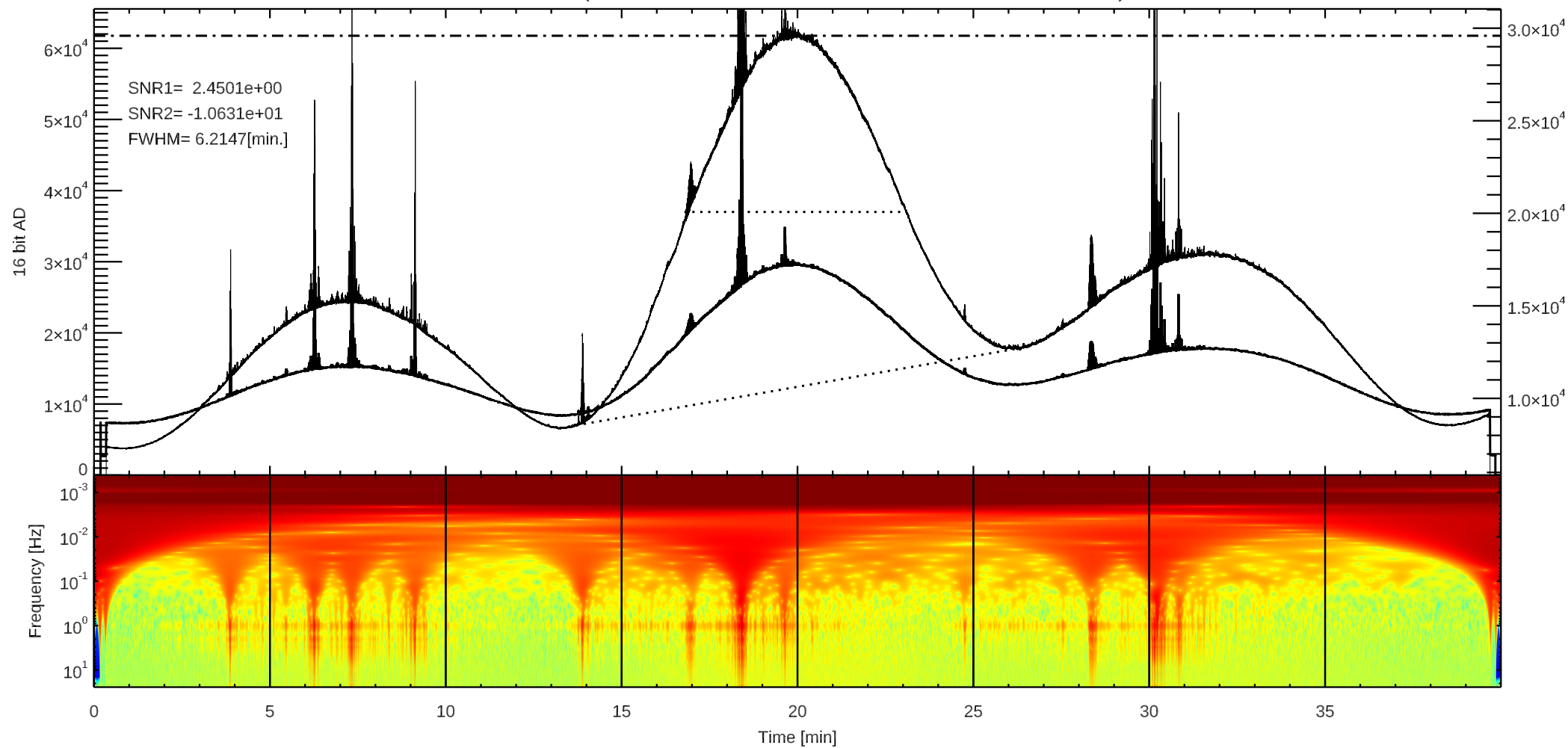
C 3C405 (/home4/archive/swift/dat/2025/09/T20250921192839.dat)
