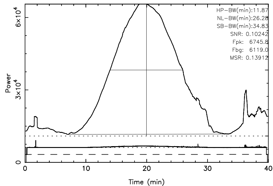
TOYOKAWA 3C10 2025/09/01(244)01:16:57–01:56:57JST
