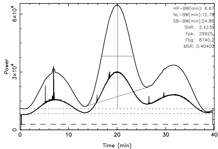
TOYOKAWA 3C405 2025/09/01(244)20:47:15–21:27:15JST
