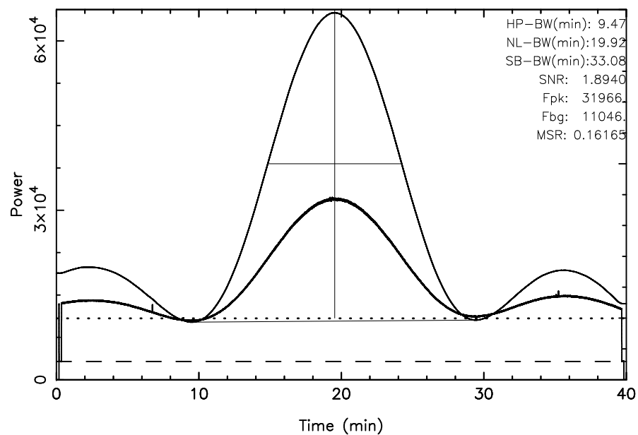
TOYOKAWA 3C461 2025/09/01(244)00:14:48–00:54:48JST
