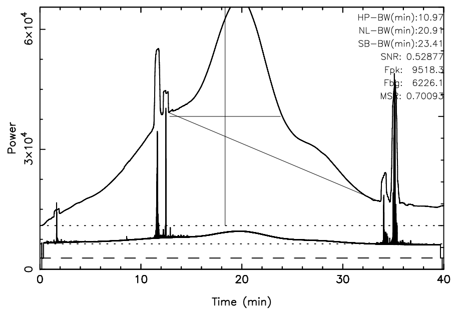
TOYOKAWA 3C392 2025/09/01(244)19:44:27–20:24:27JST
