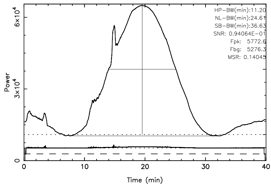
TOYOKAWA 3C10 2025/09/12(255)00:33:42-01:13:42JST
