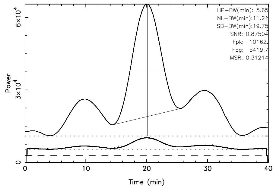
TOYOKAWA 3C144 2025/09/20(263)05:10:36-05:50:36JST
