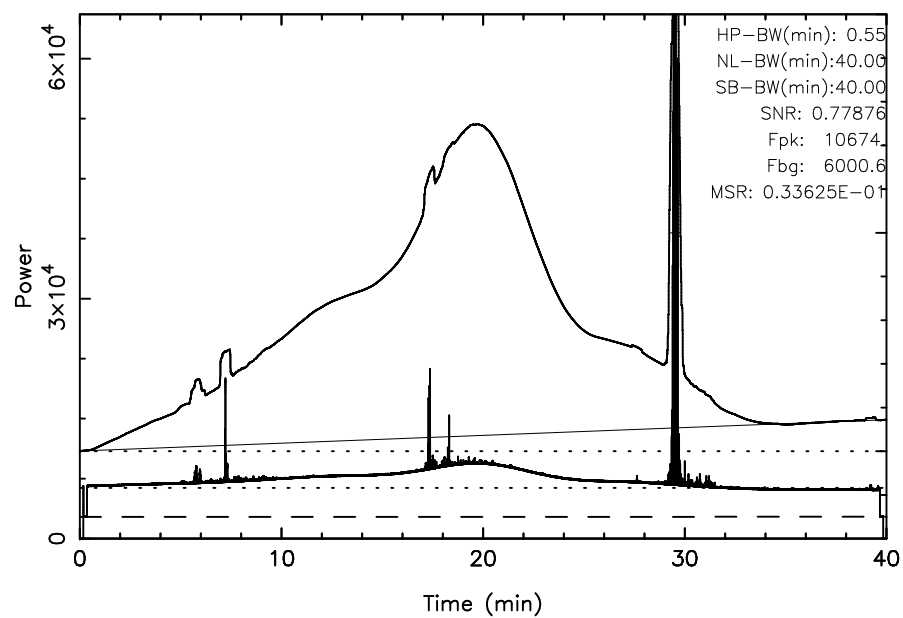
TOYOKAWA 3C392 2025/09/20(263)18:29:45-19:09:45JST
