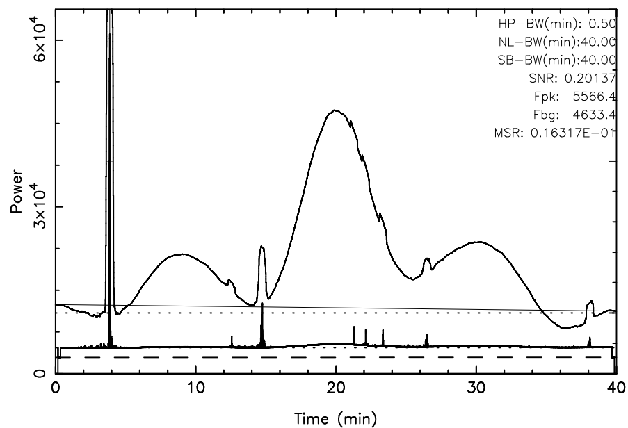
TOYOKAWA 3C123 2025/09/20(263)04:13:24-04:53:24JST
