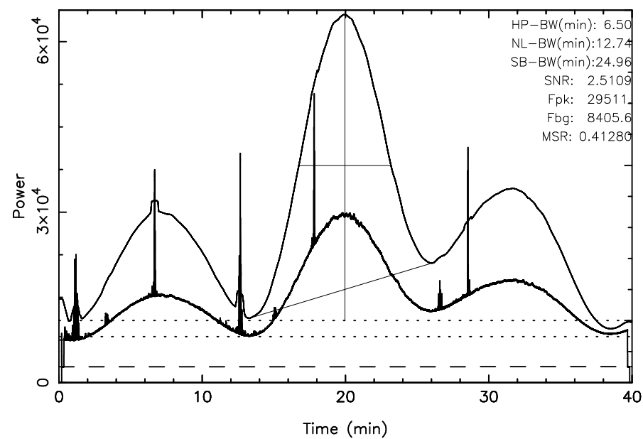
TOYOKAWA 3C405 2025/09/20(263)19:32:33-20:12:33JST
