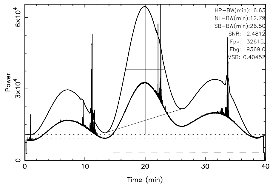
TOYOKAWA 3C405 2025/09/22(265)19:24:41-20:04:41JST
