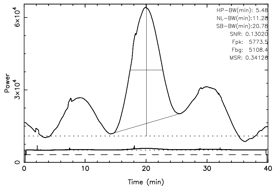
TOYOKAWA 3C123 2025/09/22(265)04:05:32-04:45:32JST
