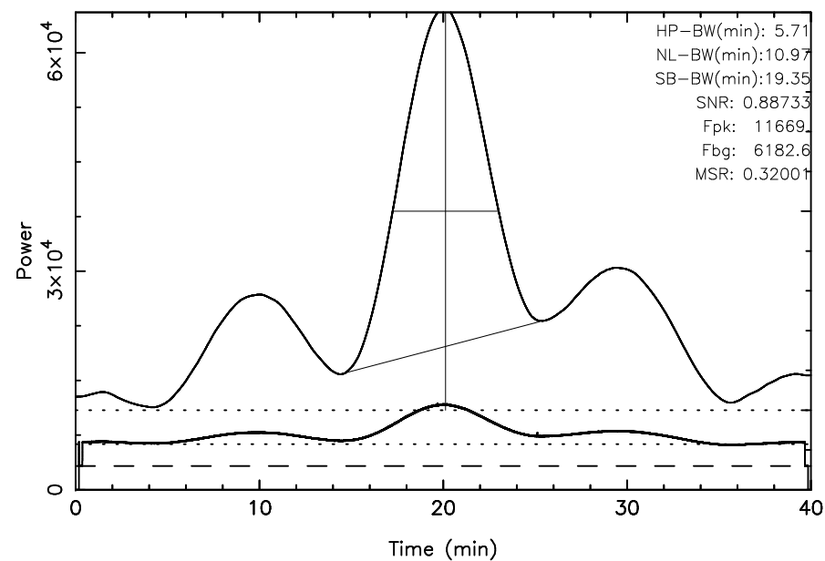
TOYOKAWA 3C144 2025/09/22(265)05:02:44-05:42:44JST
