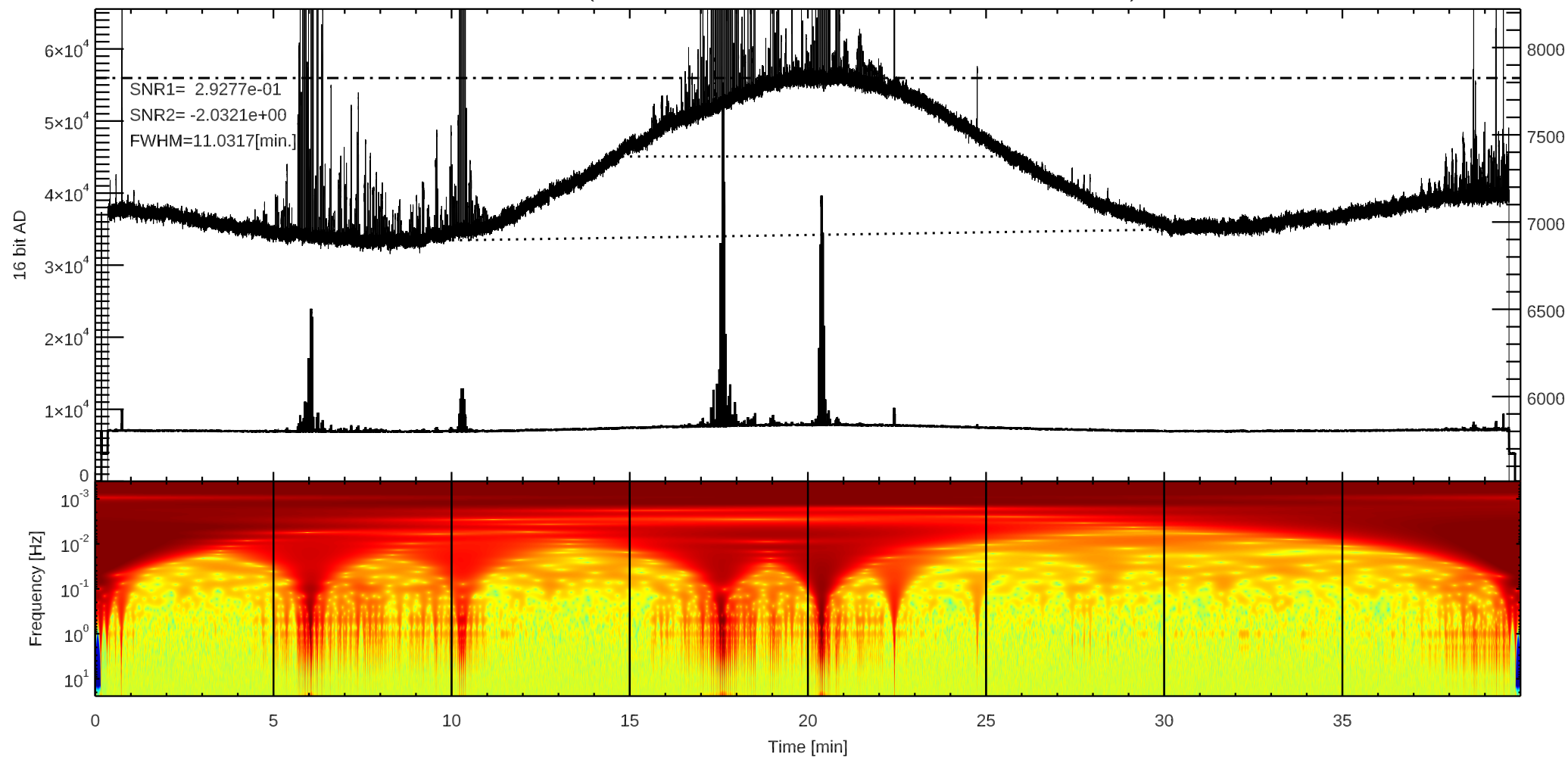
C 3C10 (/home4/archive/swift/dat/2025/10/T20251031211709.dat)
