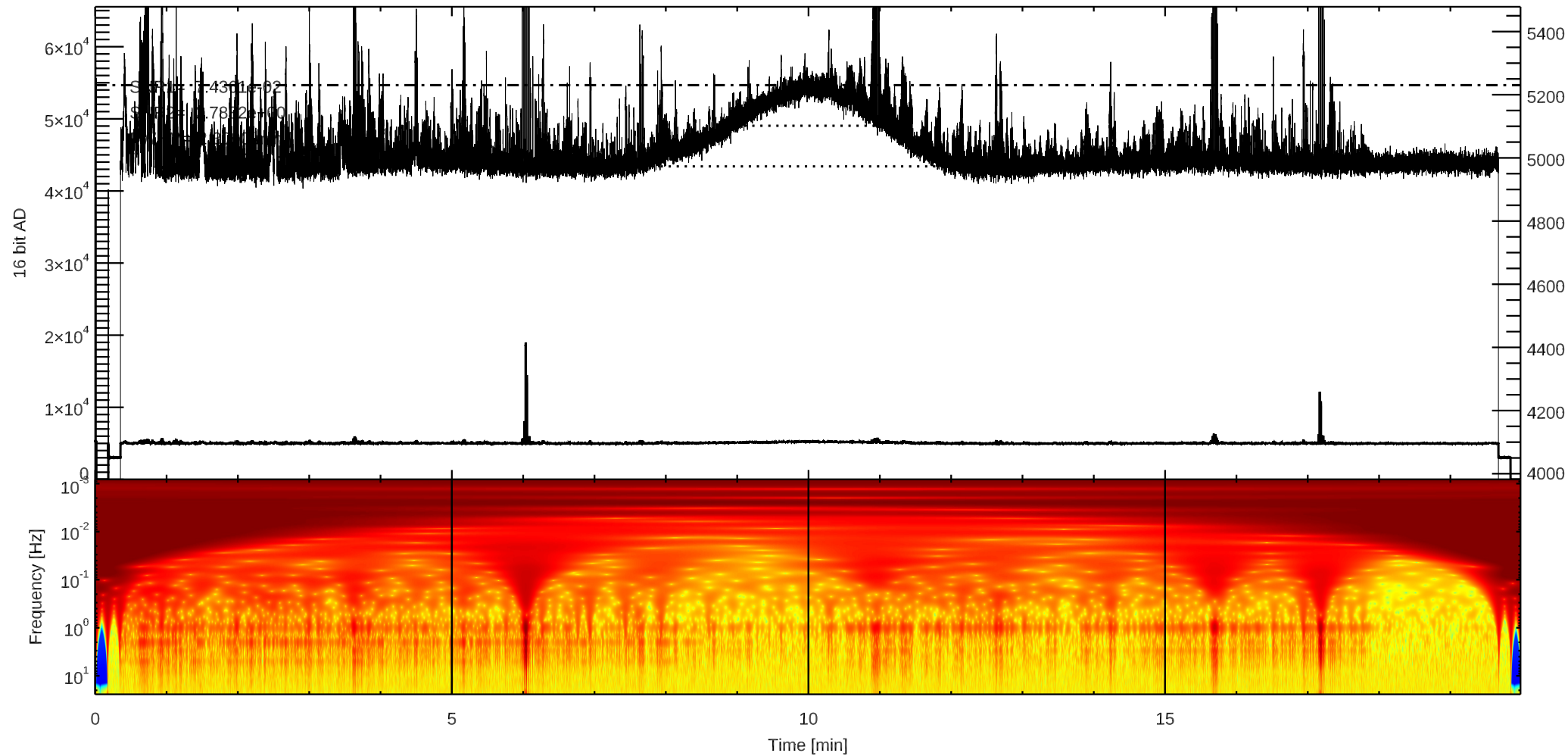
C 3C123 (/home4/archive/fit/dat/2025/10/F20251007031638.dat)
