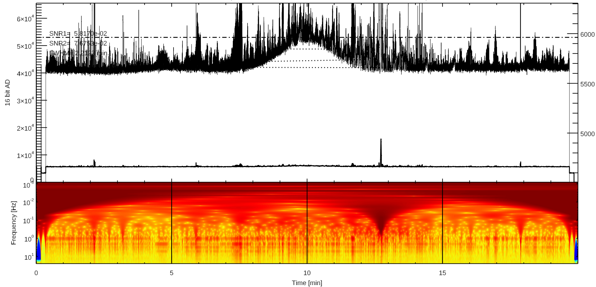
C 3C123 (/home4/archive/fit/dat/2025/10/F20251008031240.dat)
