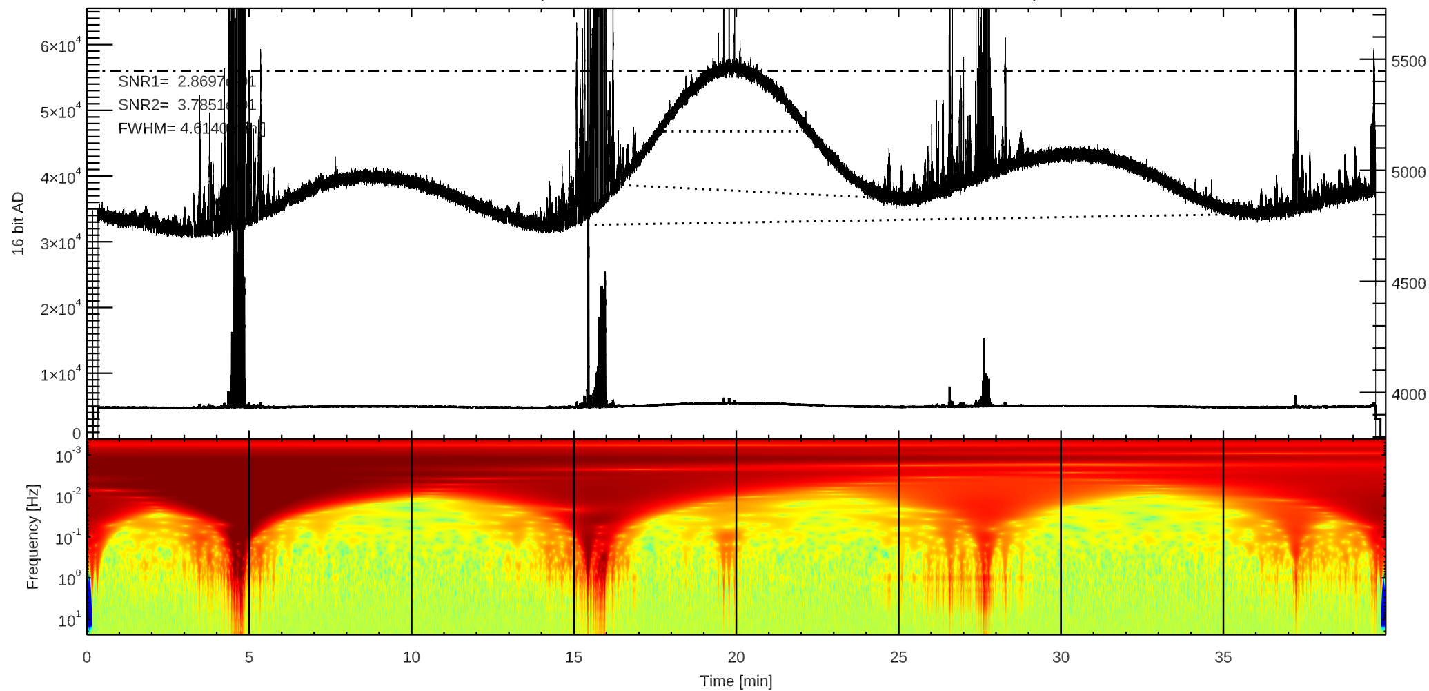
C 3C123 (/home4/archive/swift/dat/2025/10/T20251012024656.dat)
