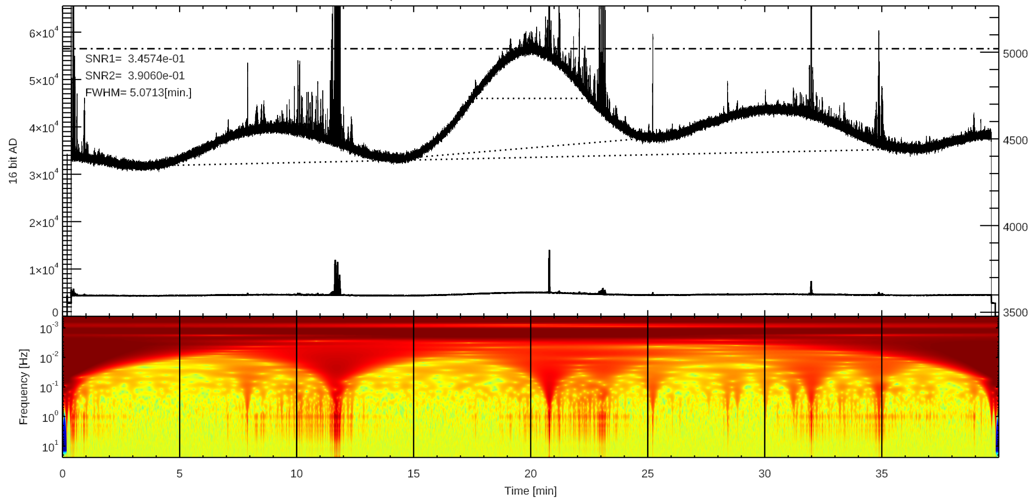
C 3C123 (/home4/archive/swift/dat/2025/10/T20251013024300.dat)
