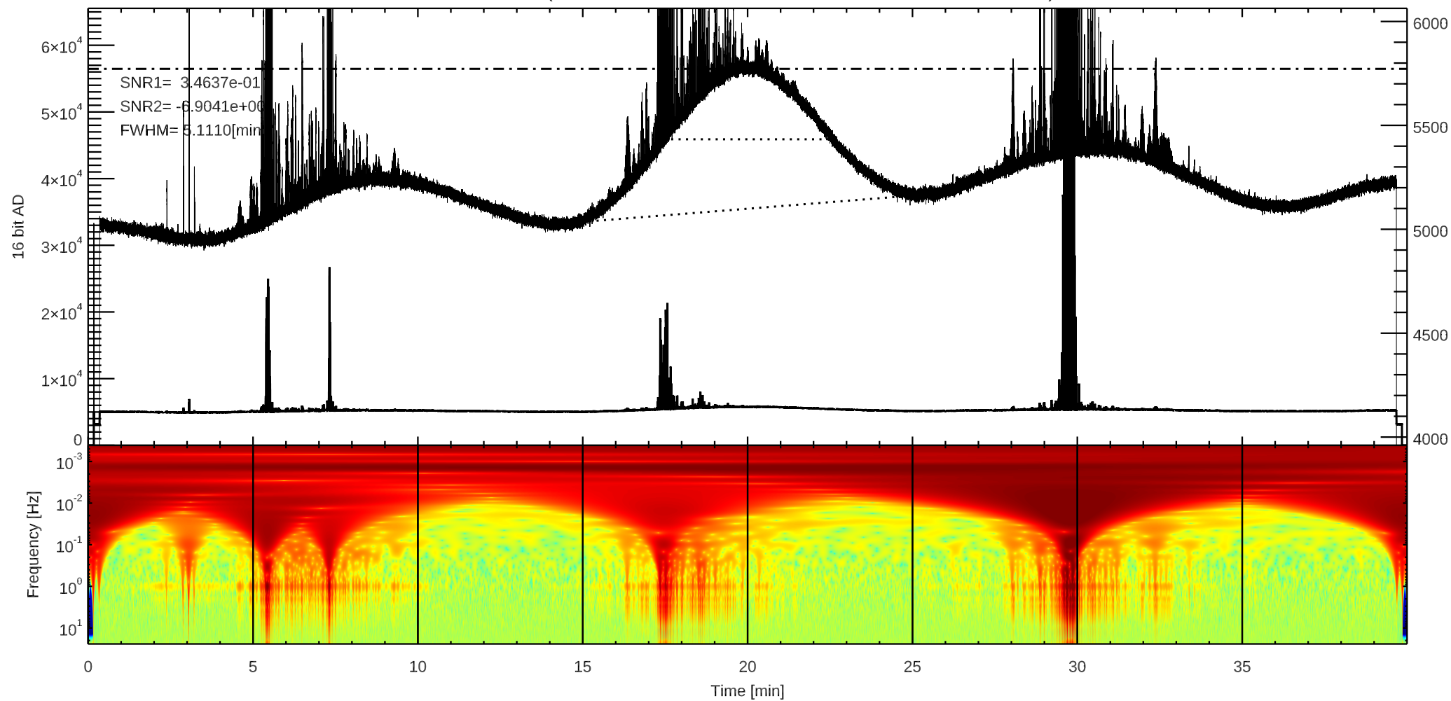
C 3C123 (/home4/archive/swift/dat/2025/10/T20251018022321.dat)
