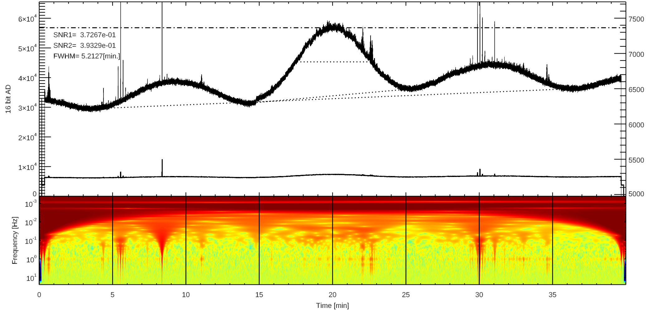
C 3C123 (/home4/archive/swift/dat/2025/10/T20251023020341.dat)
