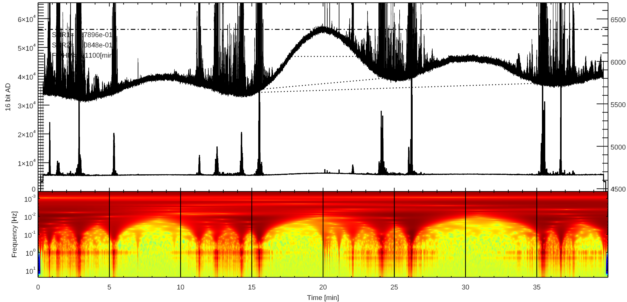
C 3C123 (/home4/archive/swift/dat/2025/10/T20251031013214.dat)
