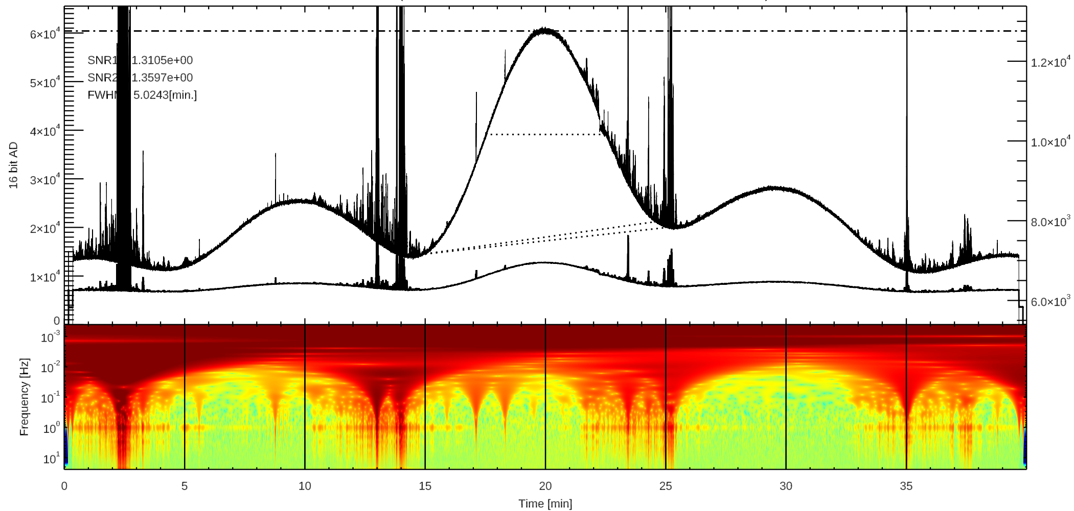
C 3C144 (/home4/archive/swift/dat/2025/10/T20251002042327.dat)
