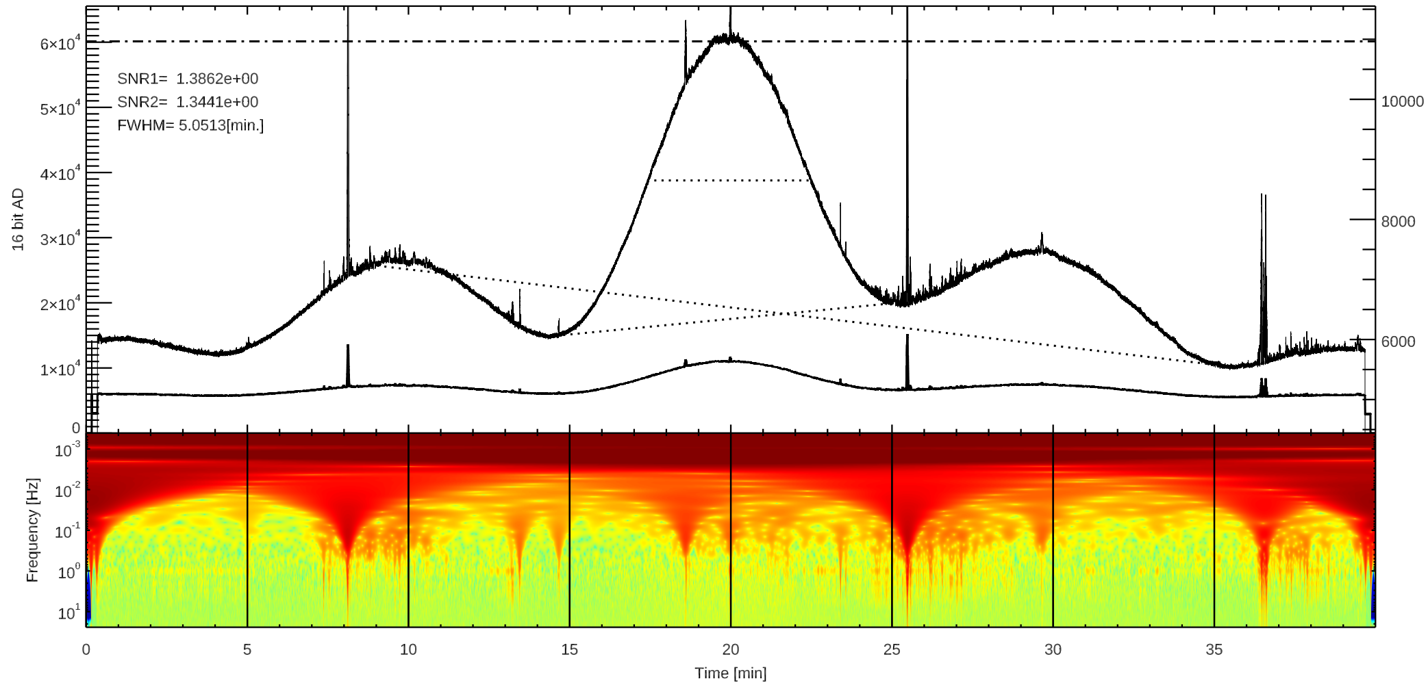
C 3C144 (/home4/archive/swift/dat/2025/10/T20251005041140.dat)
