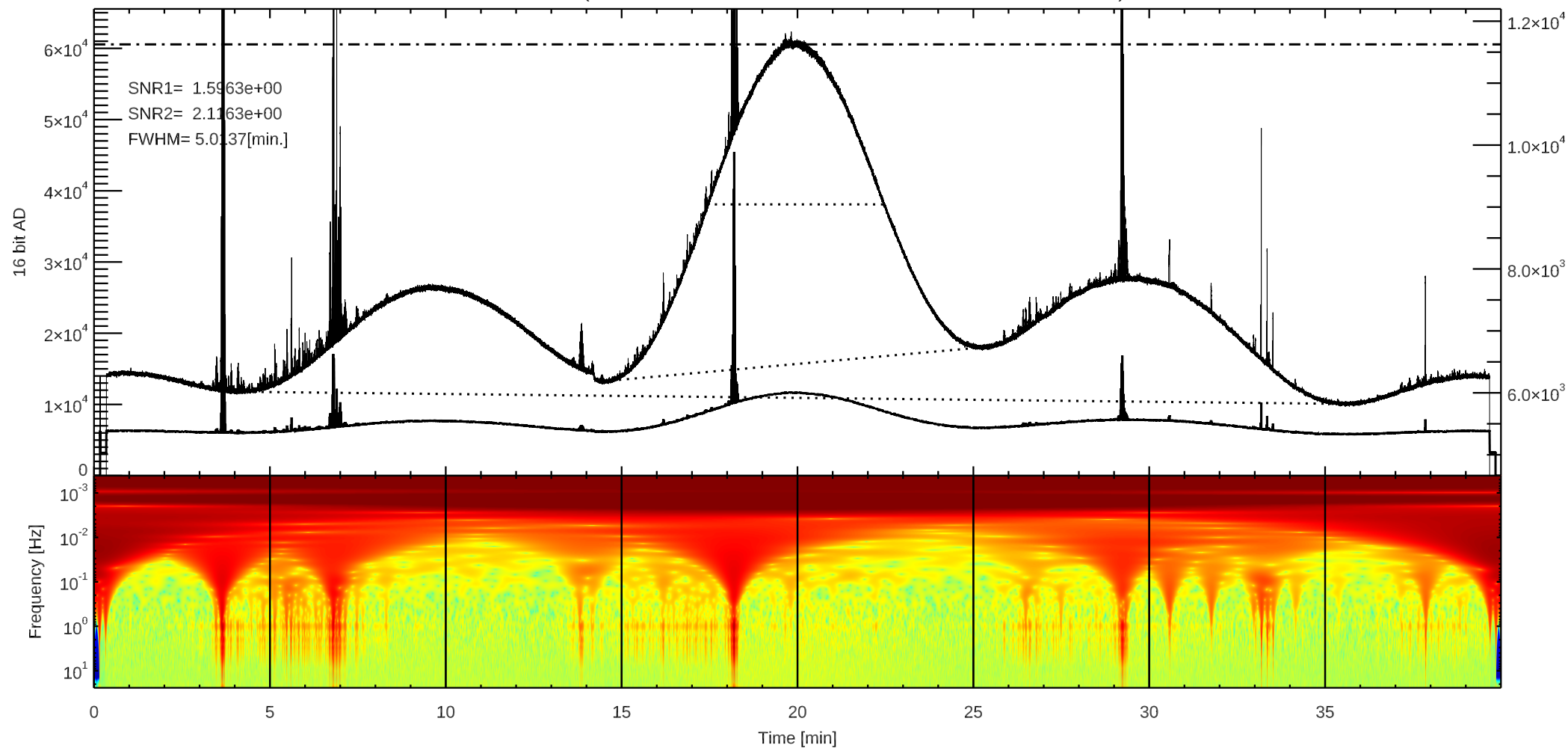
C 3C144 (/home4/archive/swift/dat/2025/10/T20251018032033.dat)
