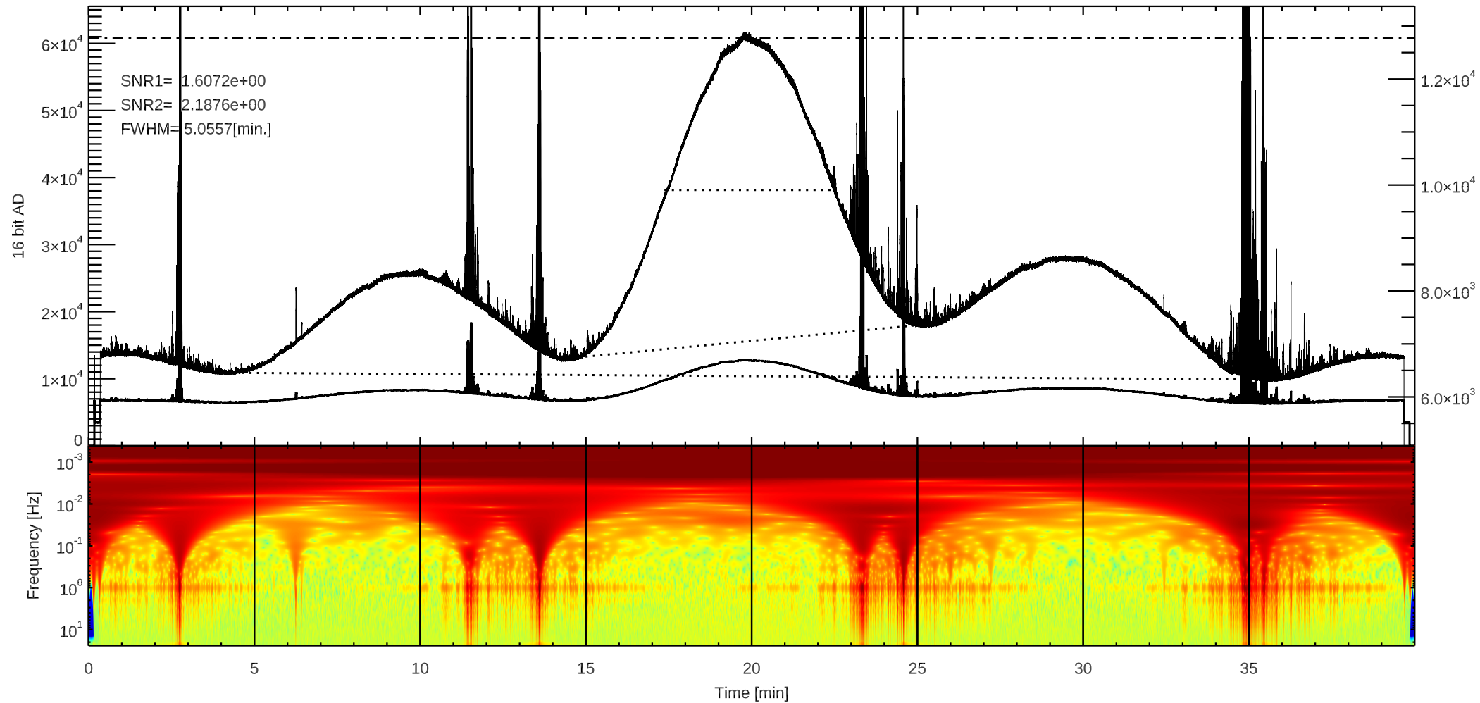
C 3C144 (/home4/archive/swift/dat/2025/10/T20251024025658.dat)
